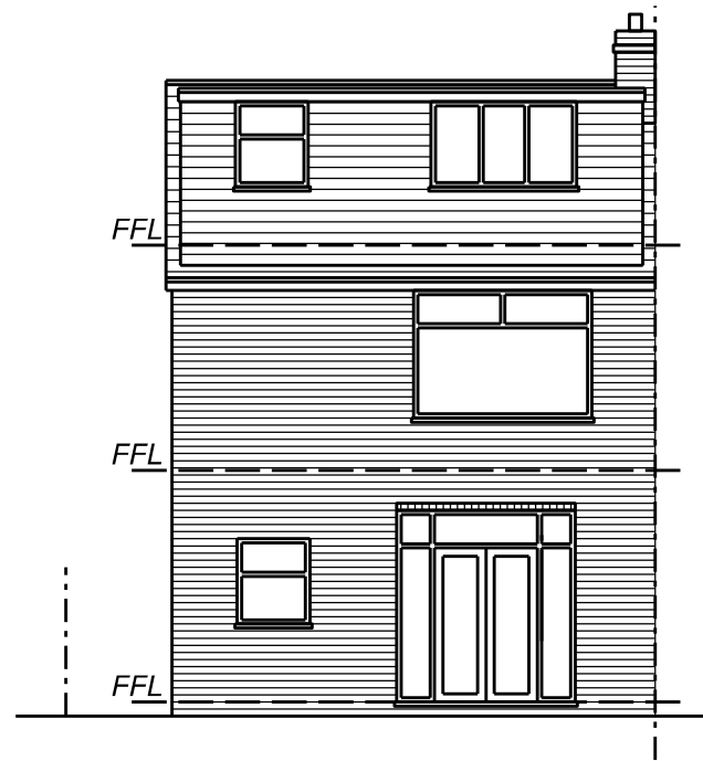
West Elevation
