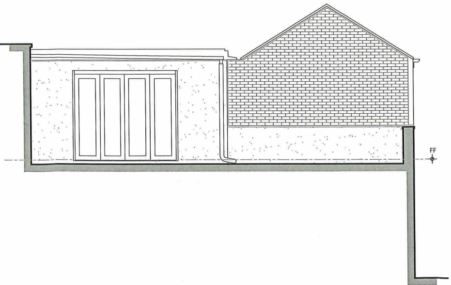
EXISTING SOUTH FACING ELEVATION SCALE - 1:100
