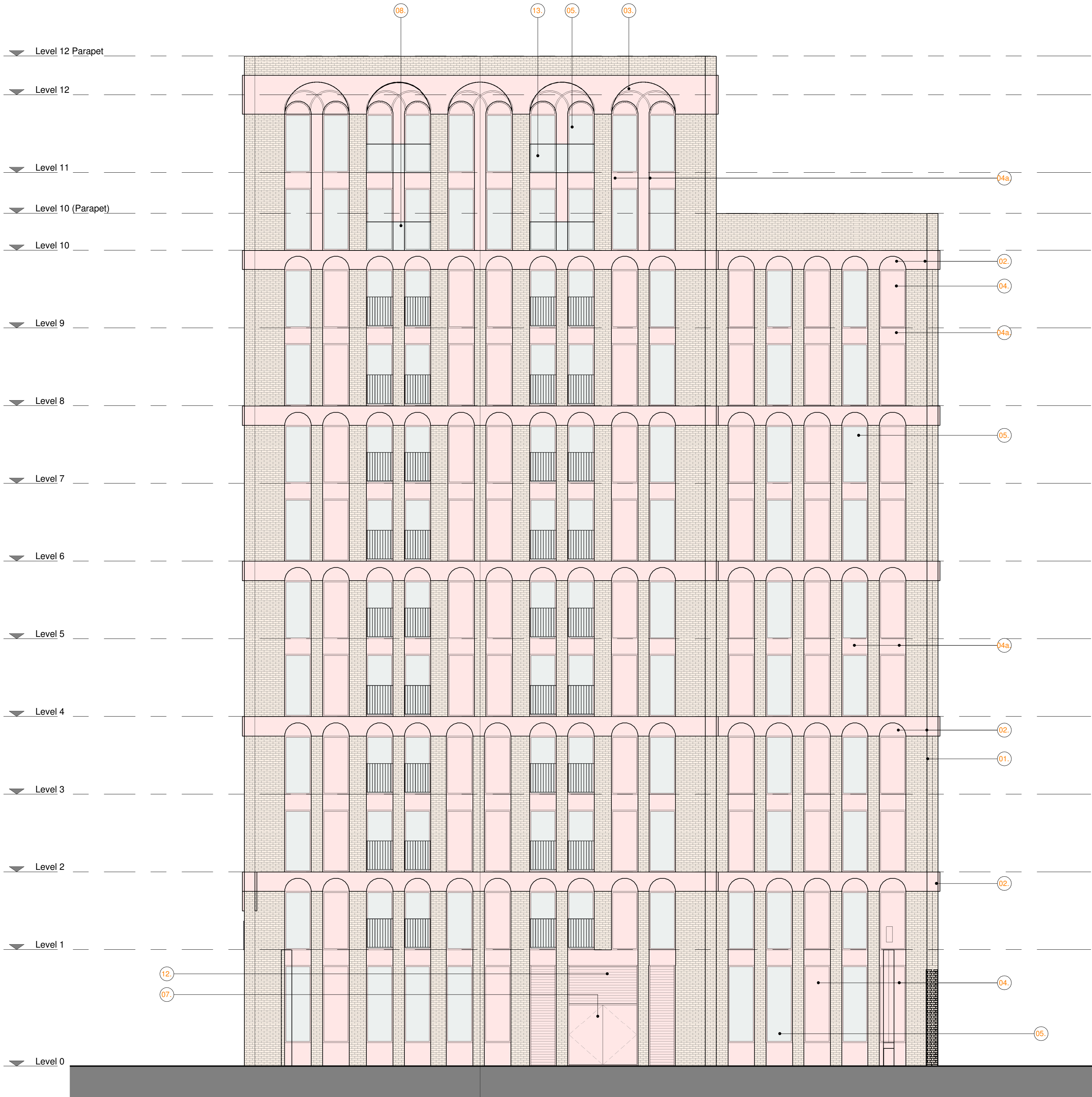
Elevation - Chadderton St 1 : 100
