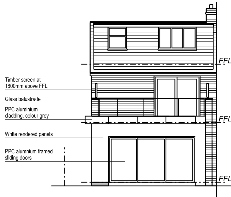
West Elevation
