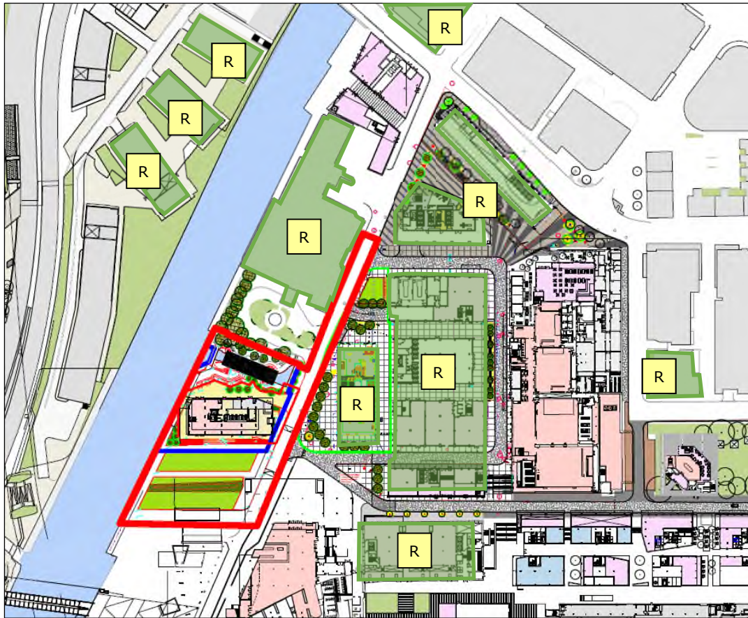
Figure 8.3A: Noise Sensitive Receptors
