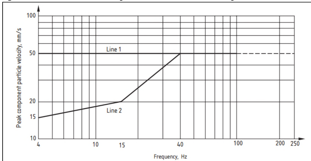
Figure 8.1A: Transient vibration guide values for cosmetic damage
