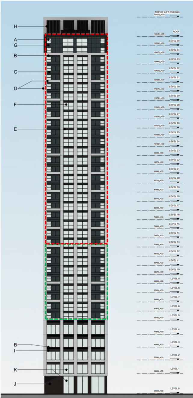
Figure 8.6A: Vision Panels to dwellings - acoustic specification location plan, west elevation
