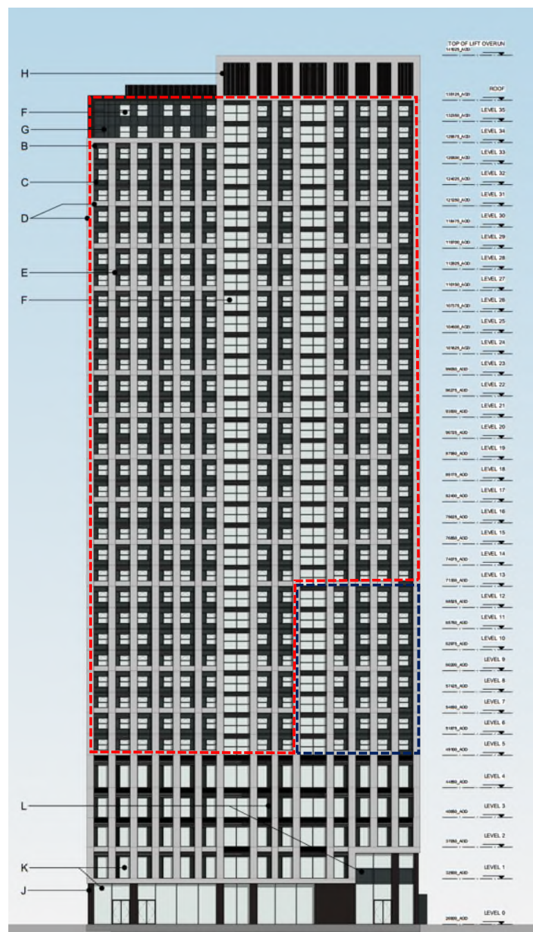
Figure 8.5A: Vision panels to dwellings-acoustic specification location plan, south elevation
