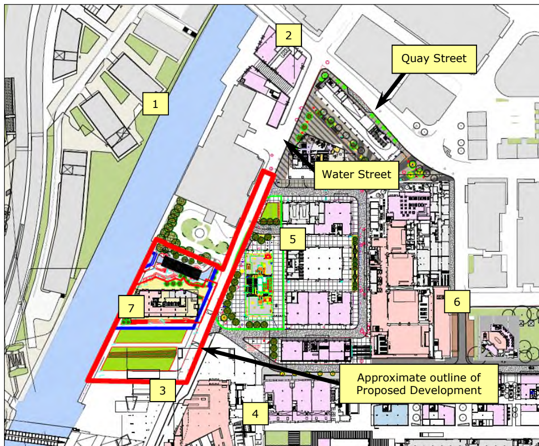
Figure 8.2A: Noise survey measurement locations
