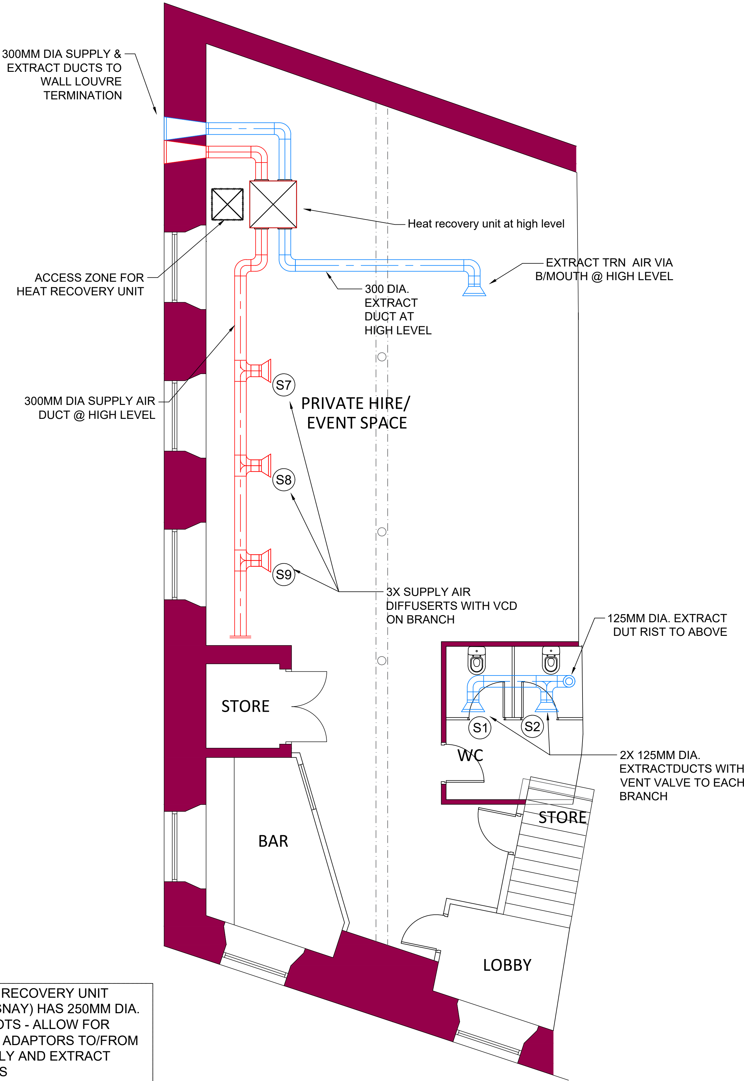
BASEMENT PLAN Scale 1:50
