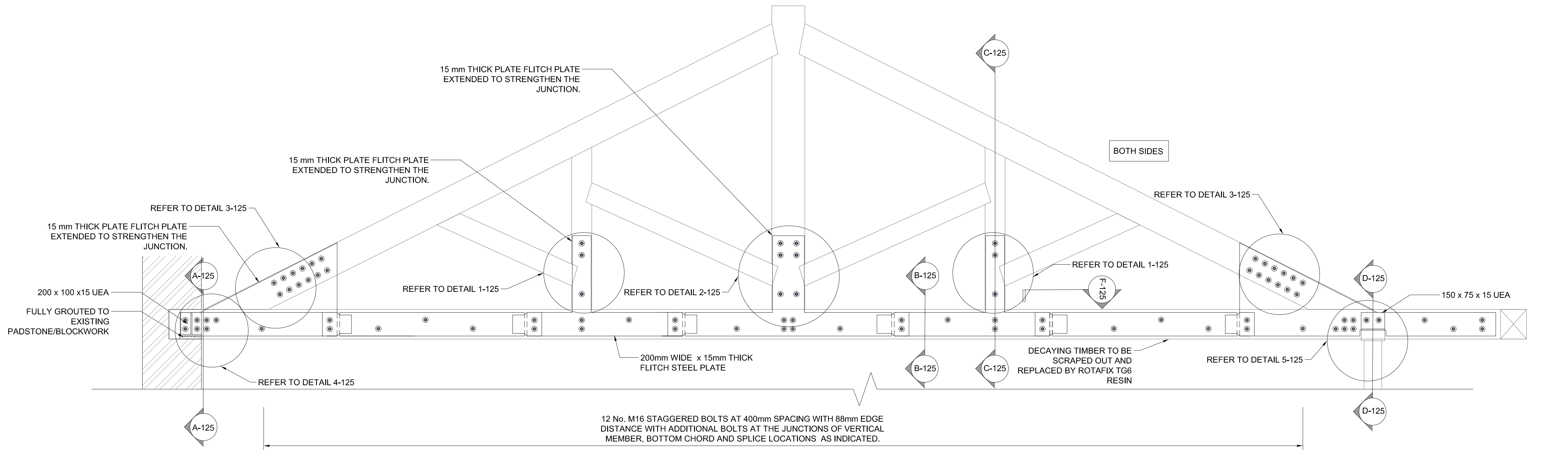
SECTION C-C ROOF TRUSS (10-T-3D) SCALE 1:20
