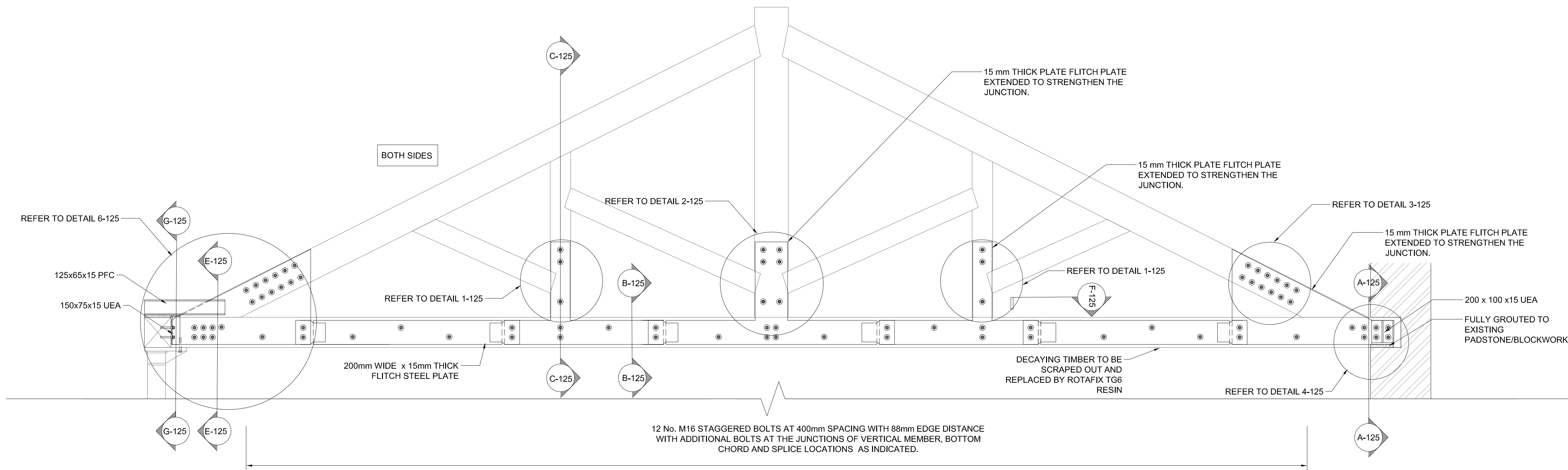
SECTION A-A ROOF TRUSS (10-T-3A) SCALE 1:20
