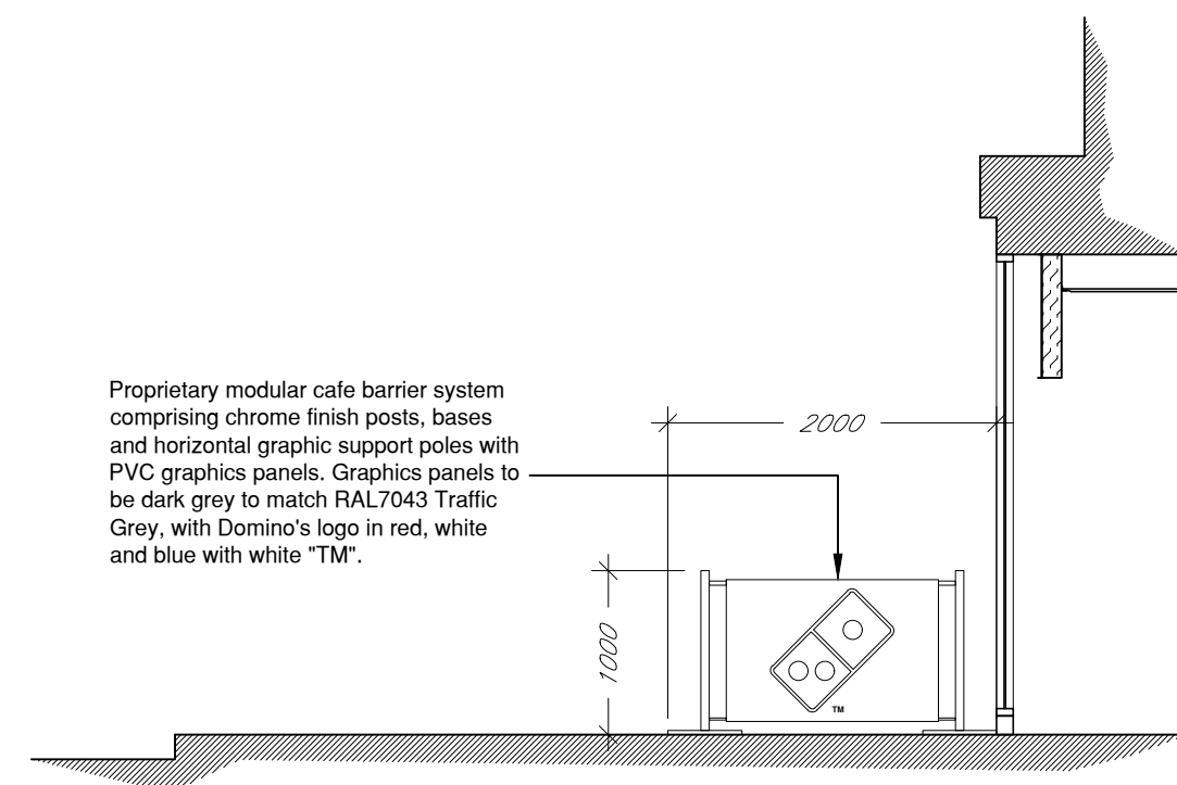
END ELEV. OF PROPOSED OUTDOOR SEATING AREA
