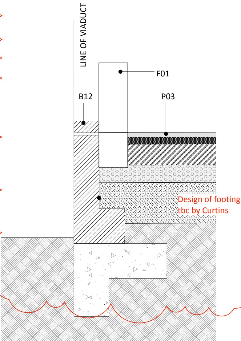
1:20 DETAIL SECTION C
