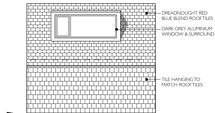
STUDIO NORTH ELEVATION (NO CHANGE TO EAST ELEVATION)
