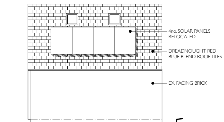
STUDIO SOUTH ELEVATION
