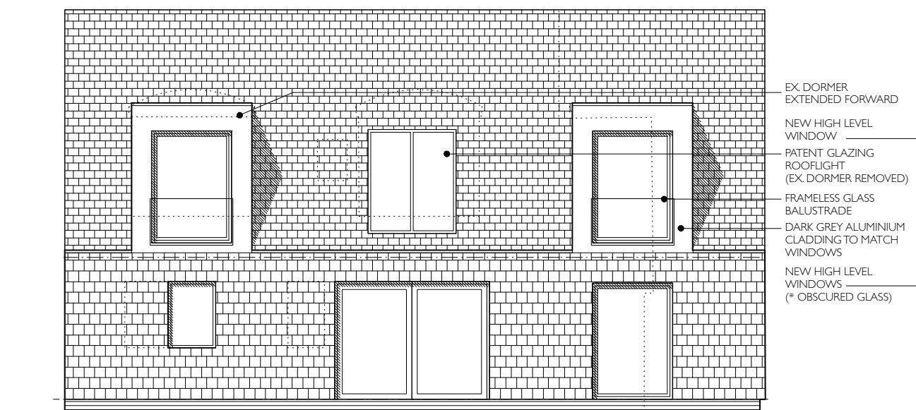
NORTH ELEVATION
