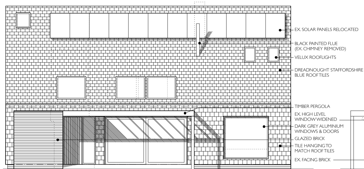
SOUTH ELEVATION
