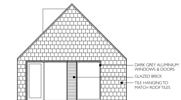
STUDIO WEST ELEVATION
