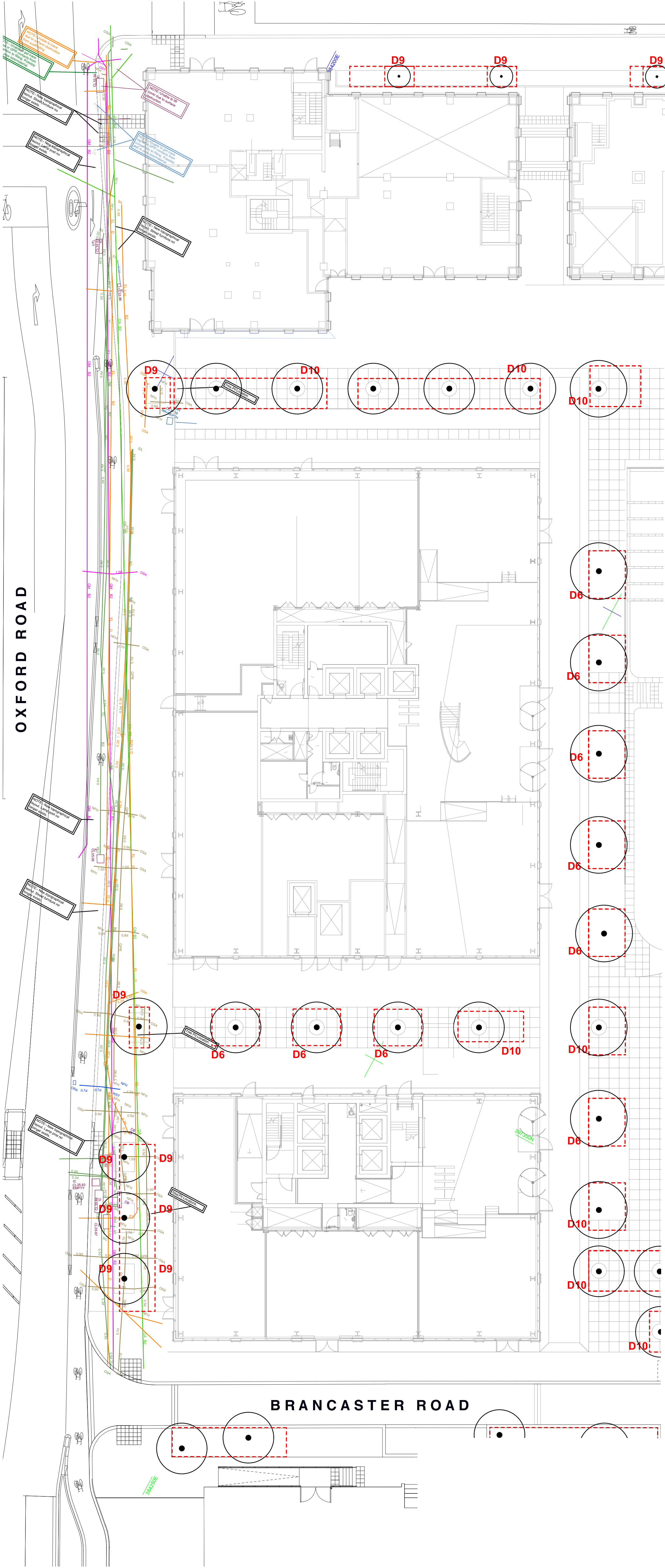
(above) B2&4 / Oxford Road Frontage Scale: 1:200 @ A1 01-11-18 FF
