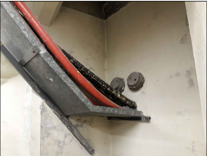
VIEW C - EXISTING HV CABLE BUILDING ENTRY (RMU ROOM 1 & 2 NOT CONSTRUCTED)
