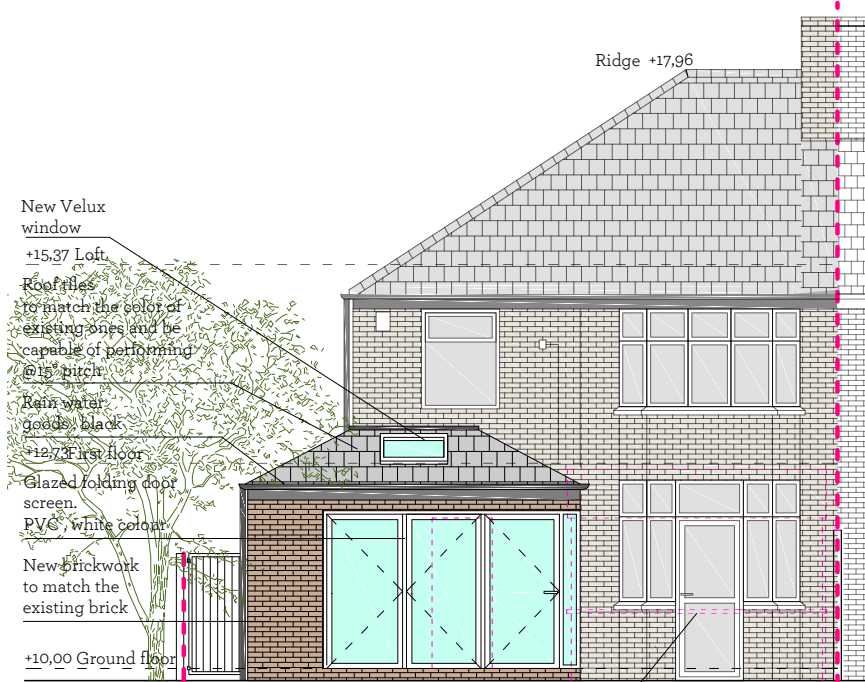
Garden elevation
