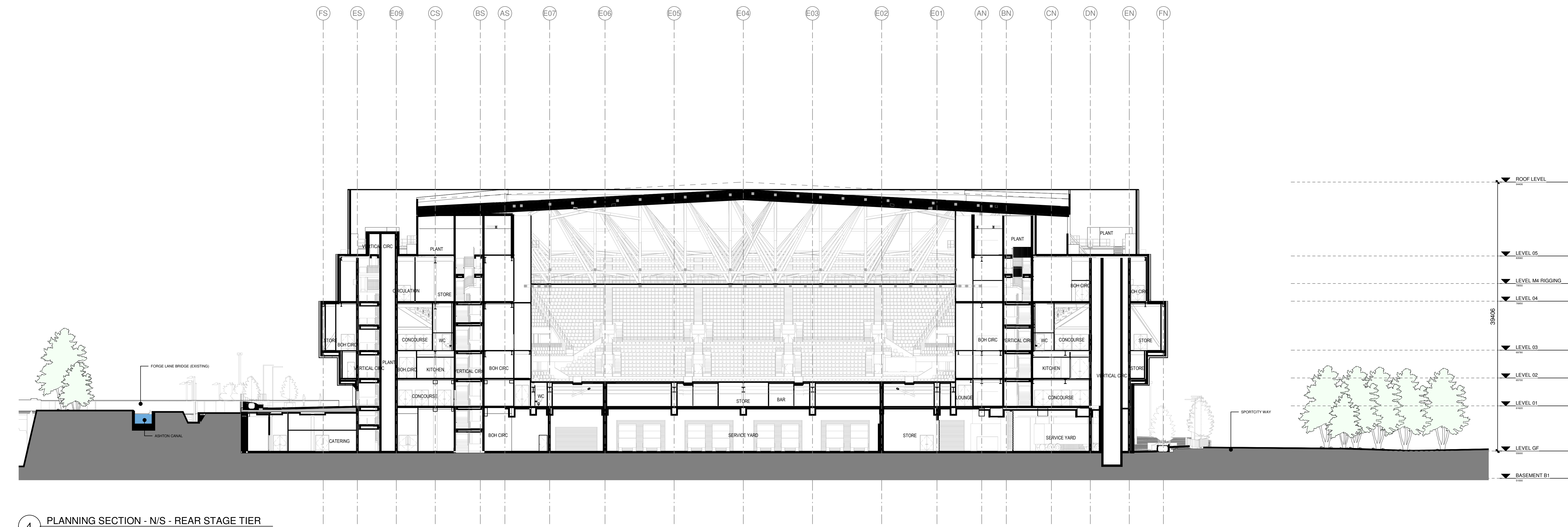
4 PLANNING SECTION - N/S - REAR STAGE TIER 1:250
