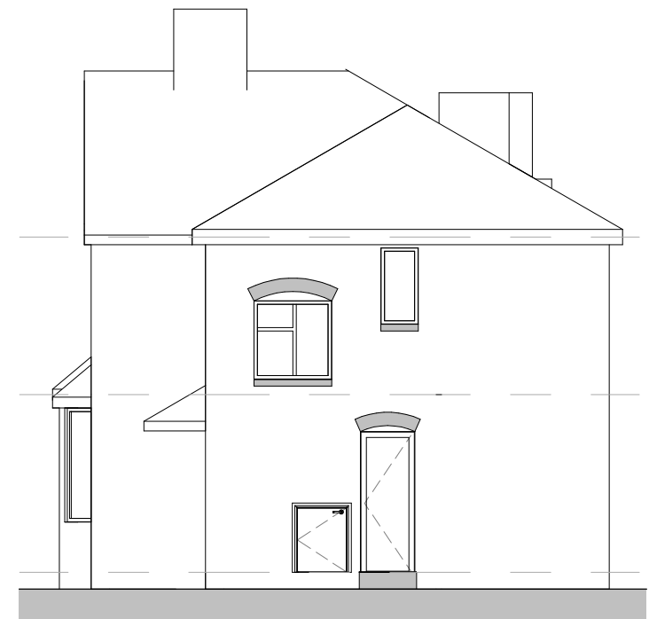
02-E-Elevation 1 : 100
