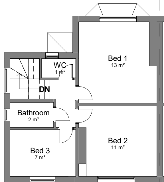
00-E-Ground Floor 1 : 100
