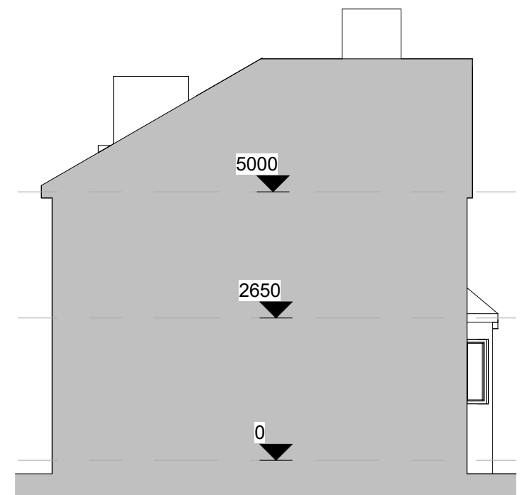
04-E-Elevation 1 : 100
