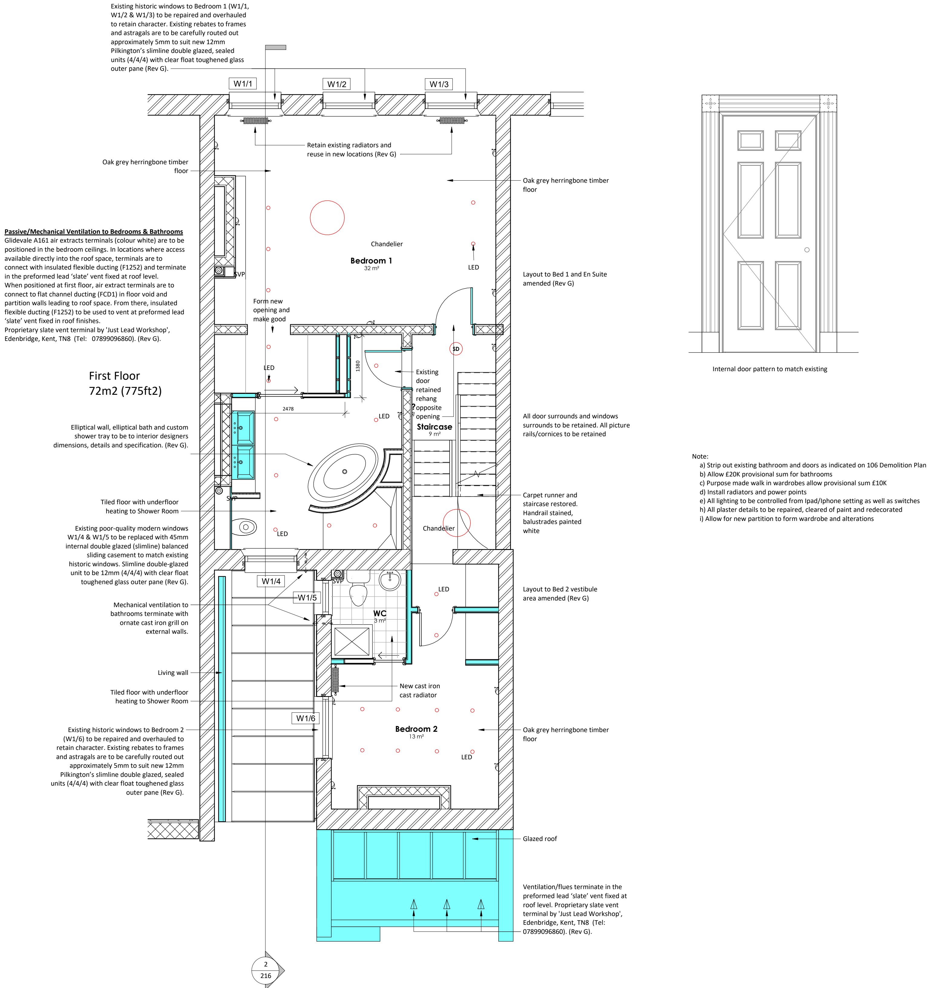
01 First Floor as Proposed 1 : 50
