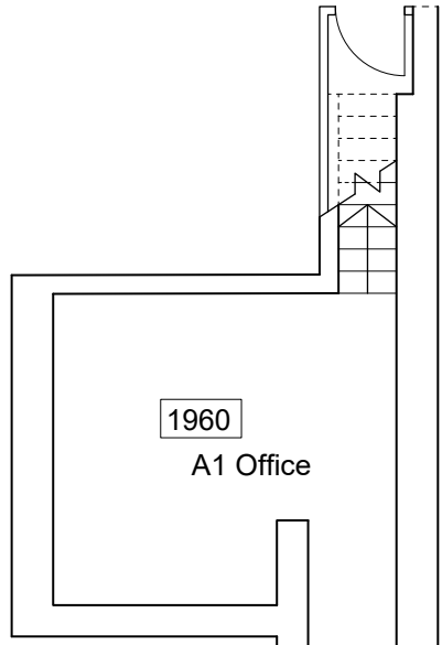
BASEMENT FLOOR SCALE 1:100 EXISTING - E003
