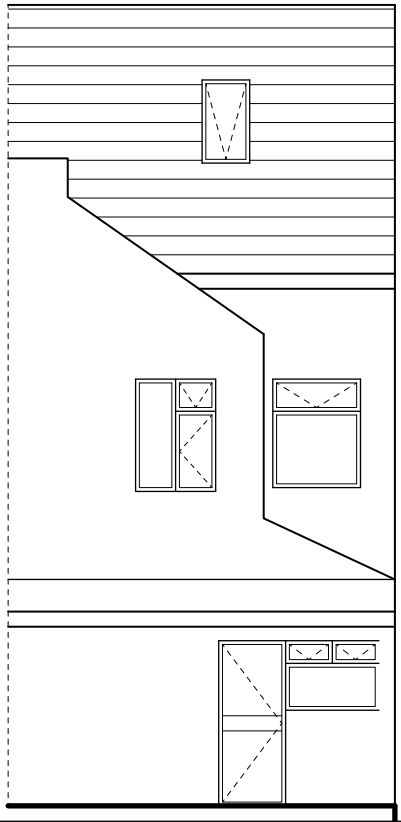
NORTH EAST ELEVATION SCALE 1:100 EXISTING - E008
