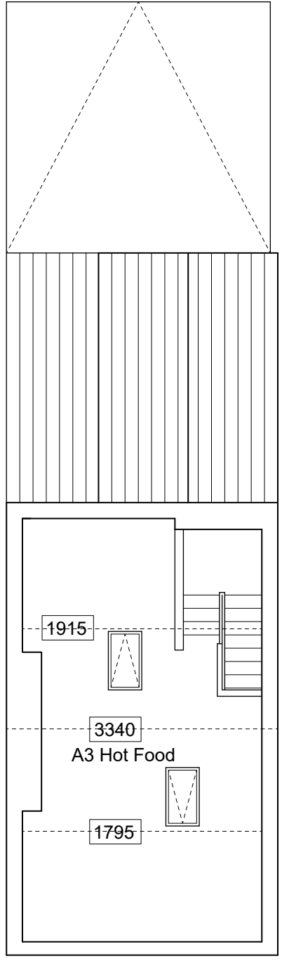
SECOND FLOOR SCALE 1:100 PROPOSED - P006
