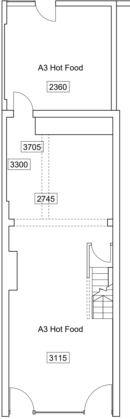
GROUND FLOOR SCALE 1:100 PROPOSED - P004
