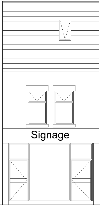
SOUTH WEST ELEVATION SCALE 1:100 EXISTING - E007
