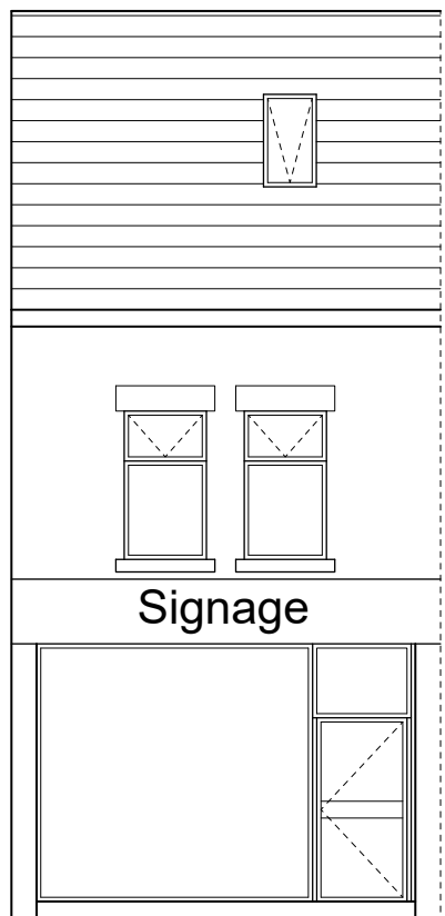
SOUTH WEST ELEVATION SCALE 1:100 PROPOSED - P007
