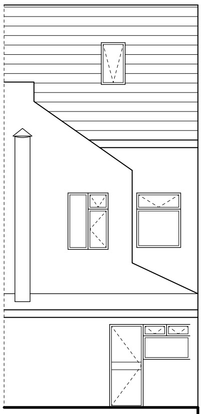
NORTH EAST ELEVATION SCALE 1:100 PROPOSED - P008
