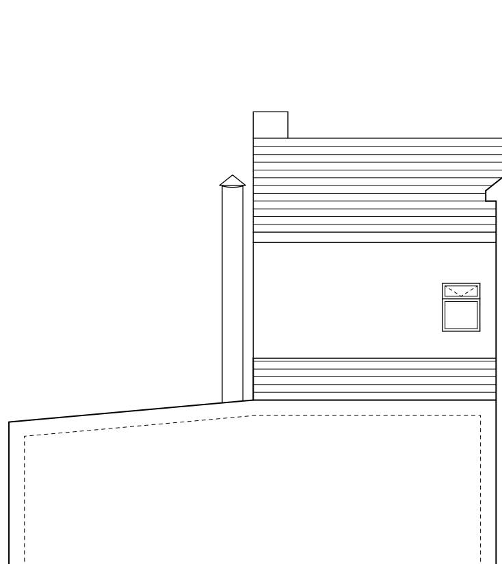
NORTH WEST ELEVATION SCALE 1:100 PROPOSED - P009
