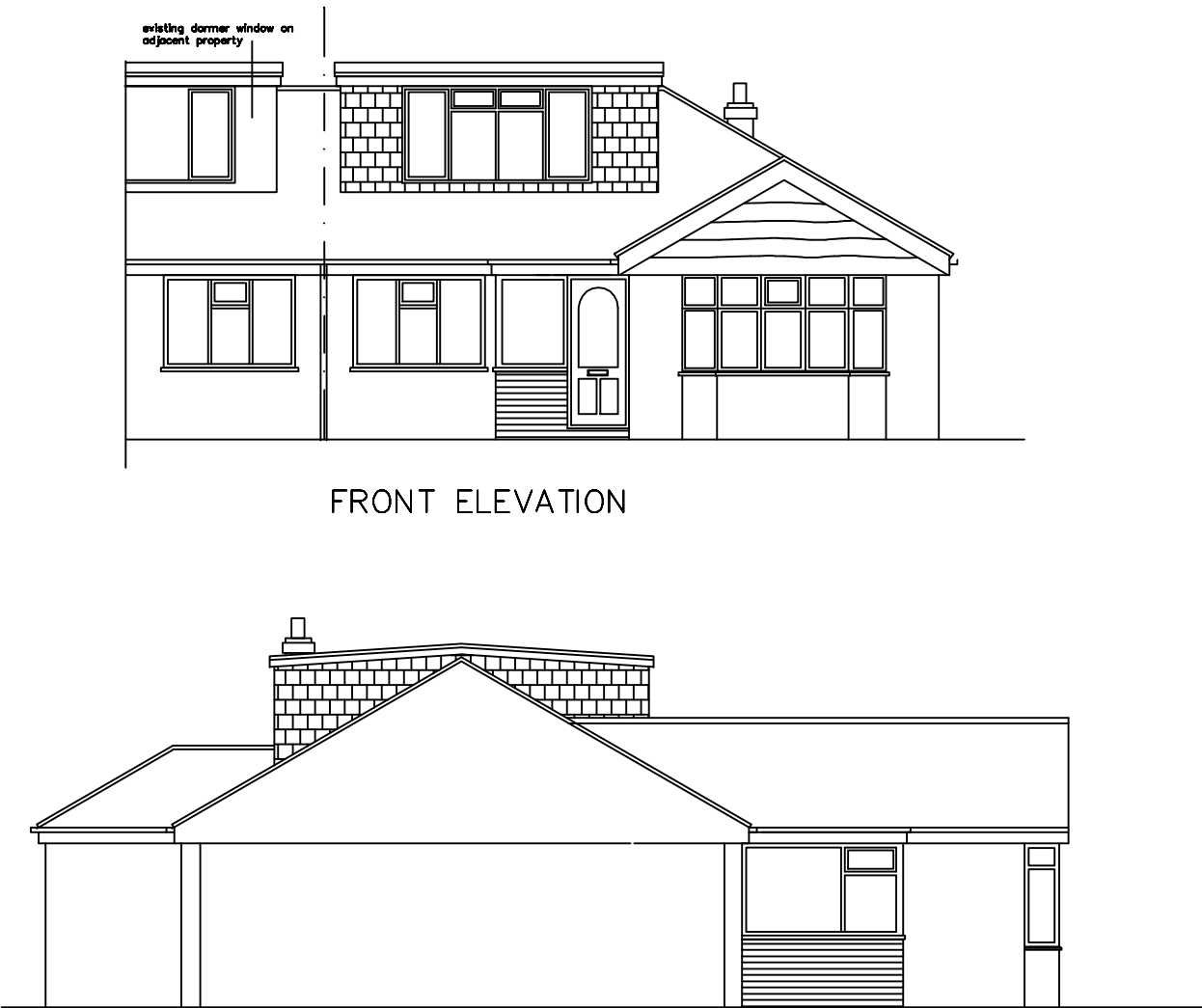
SIDE ELEVATION
