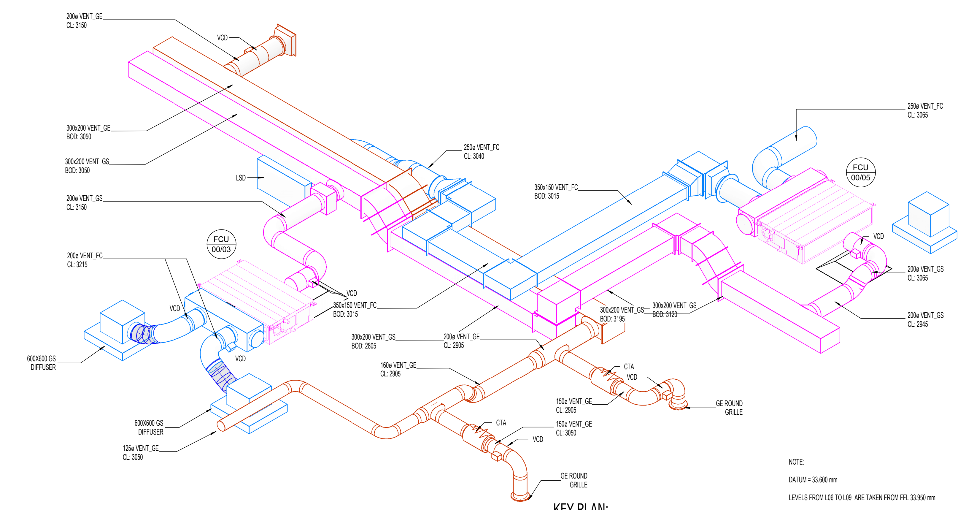
01 7L - VENTILATION - LEVEL GROUND FLOOR - 3D VIEW 01
