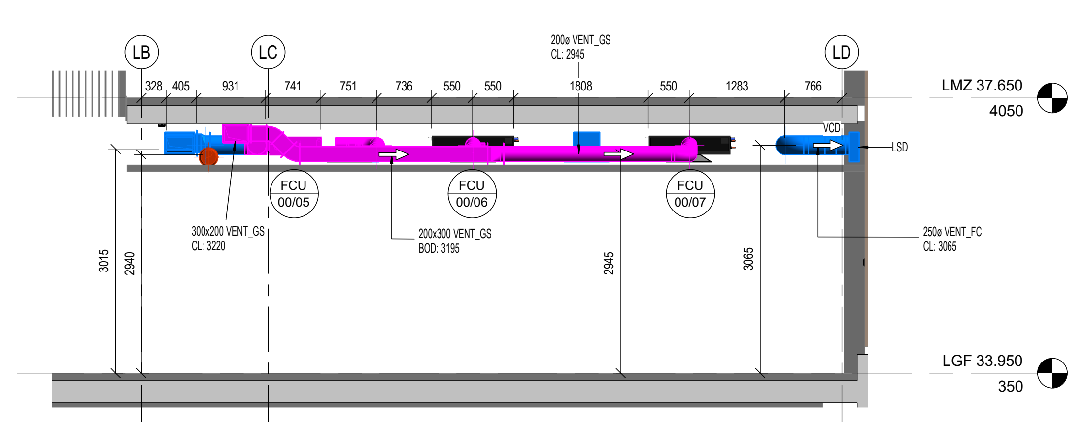
A 7L - VENTILATION - LEVEL GROUND FLOOR - SECTION A 1:50
