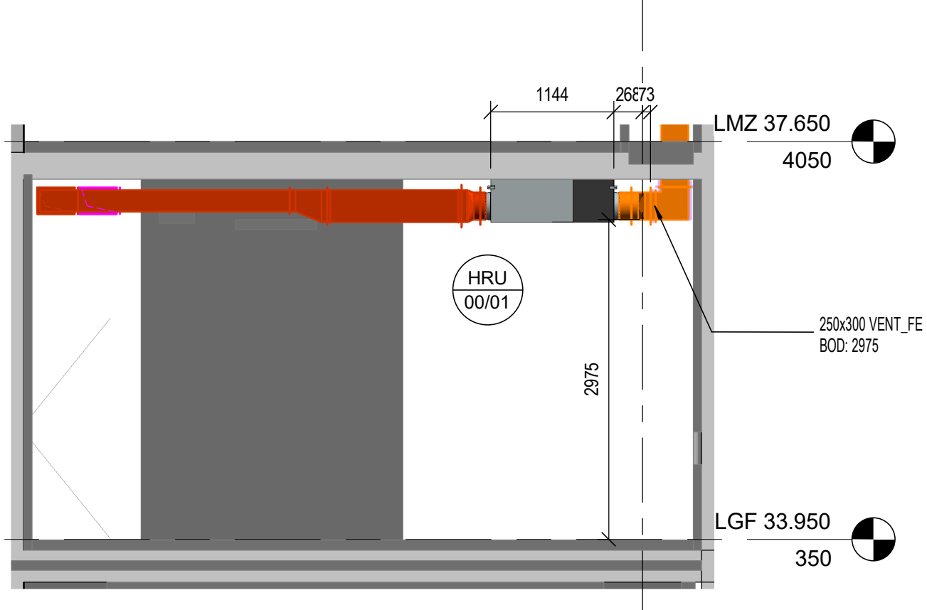
C 7L - VENTILATION - LEVEL GROUND FLOOR - SECTION C 1:50
