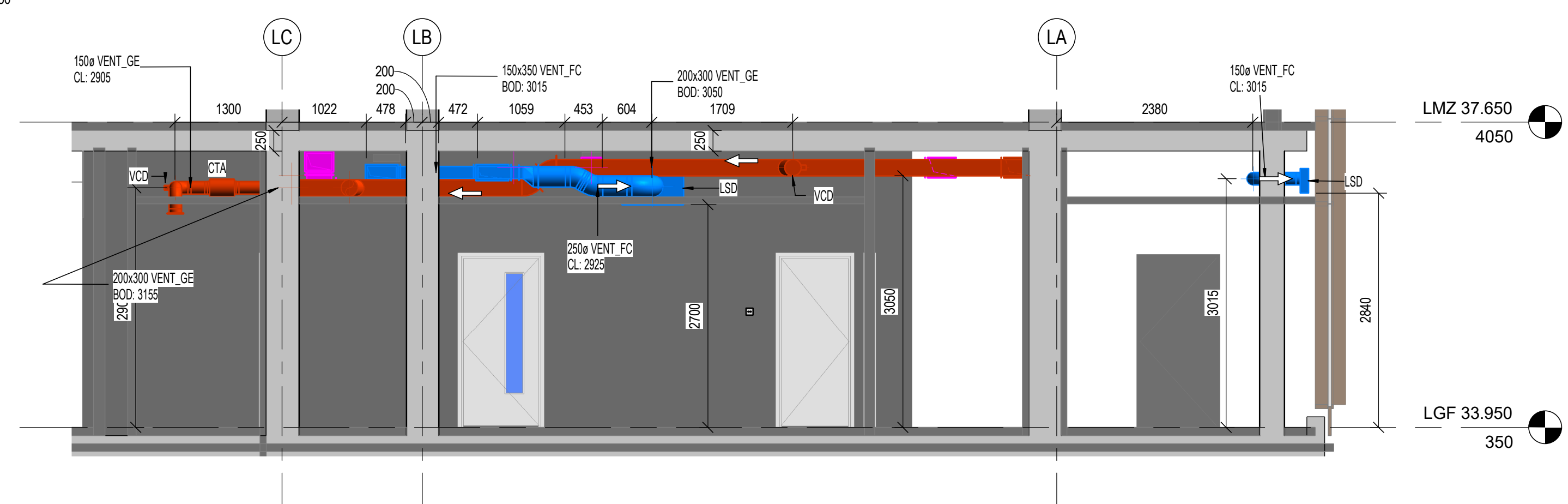
A 7L - VENTILATION - LEVEL GROUND FLOOR - SECTION A 1:50
