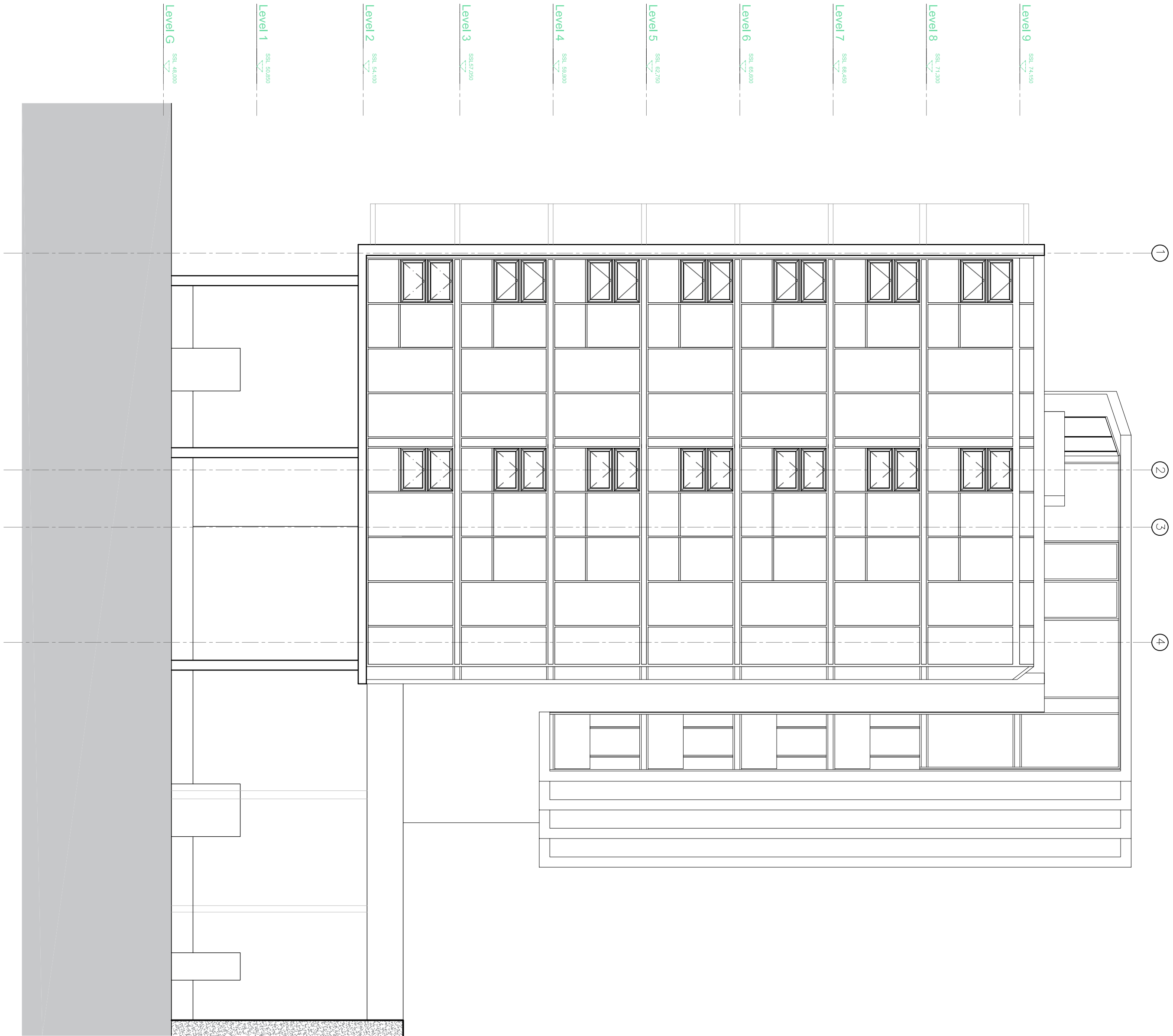
BLOCK A - Elevation B as existing
