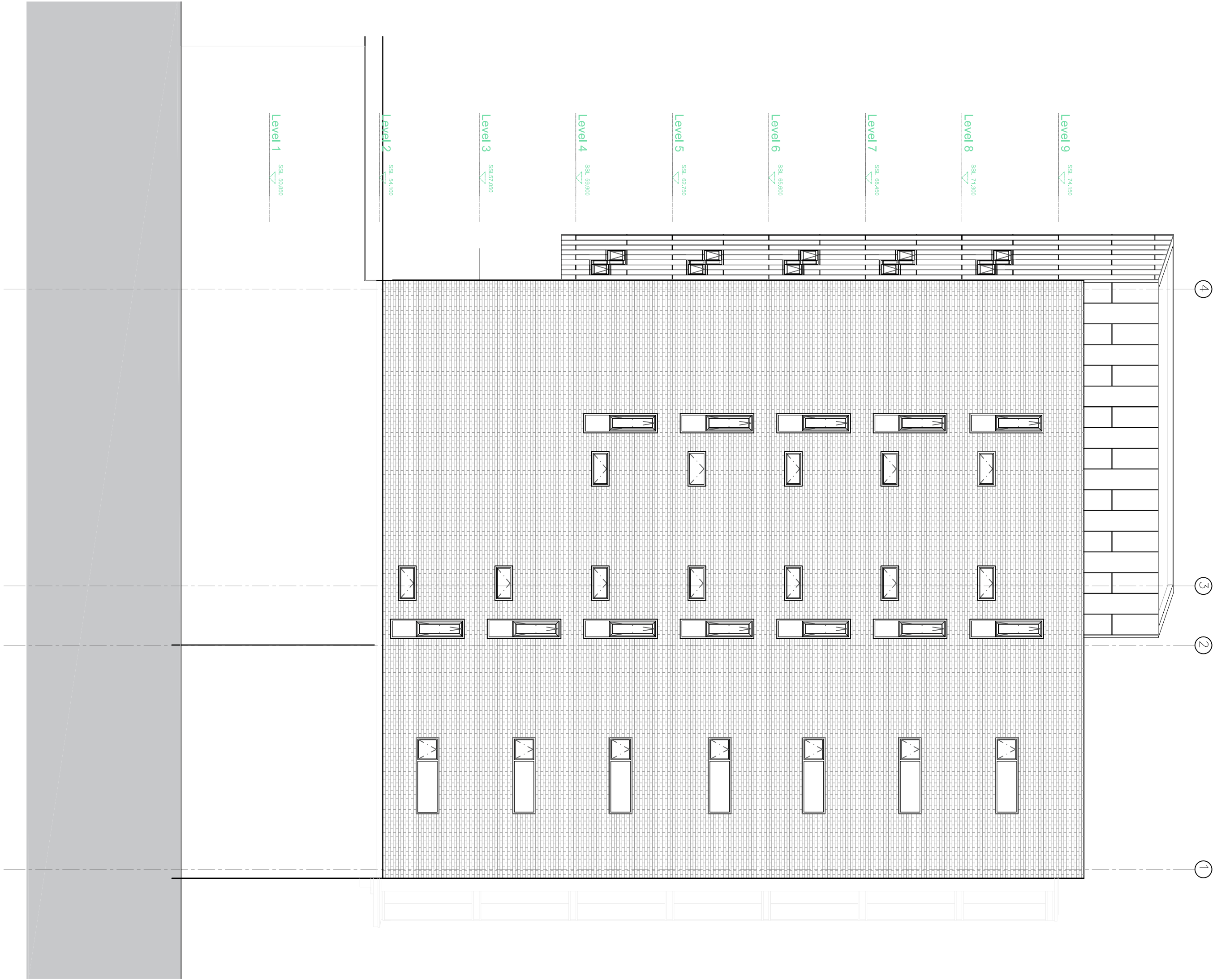
BLOCK A - Elevation D as existing
