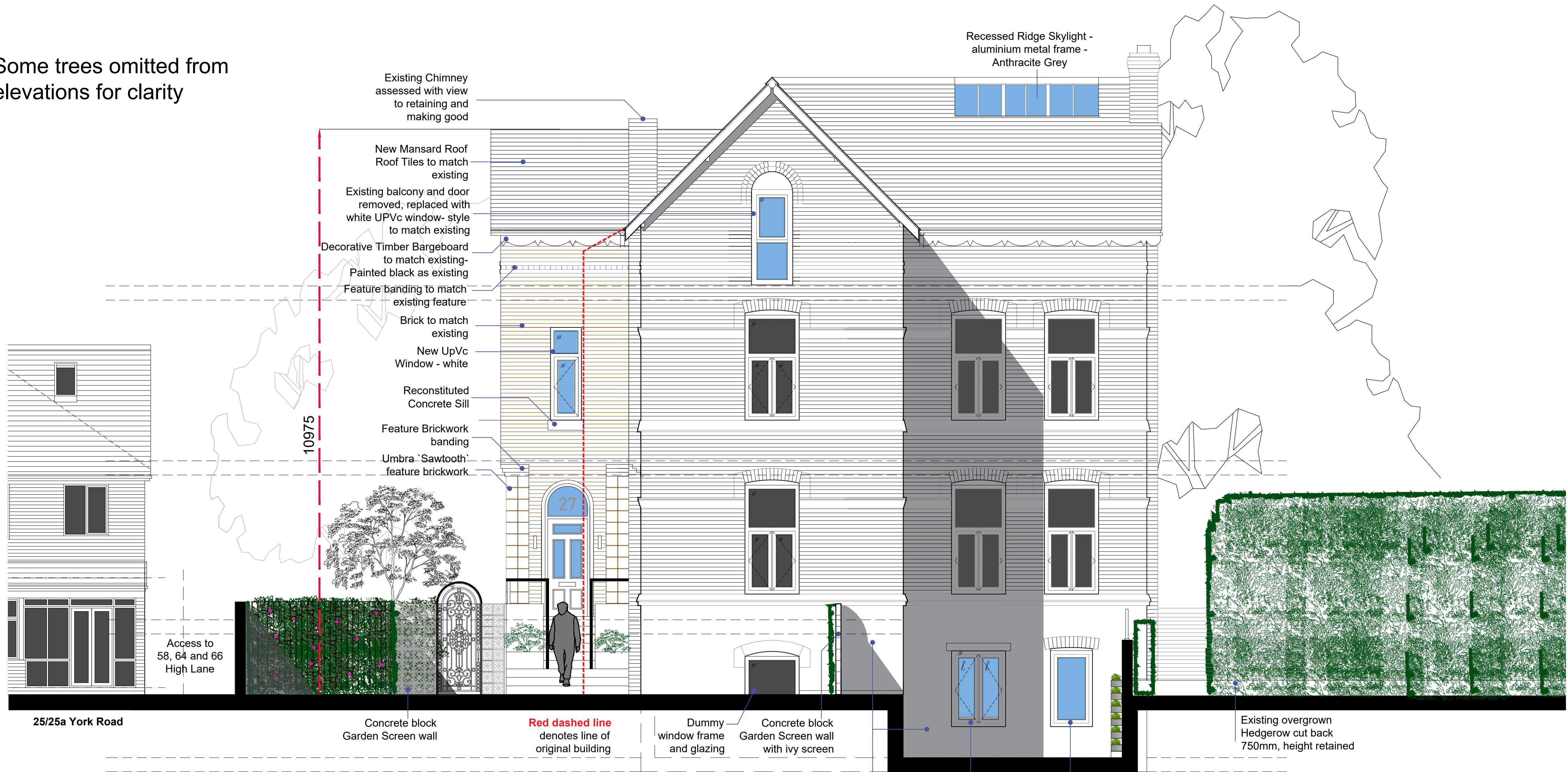
Proposed York Road Elevation 1:50
