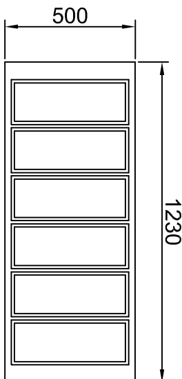
Type E - 2no Required
