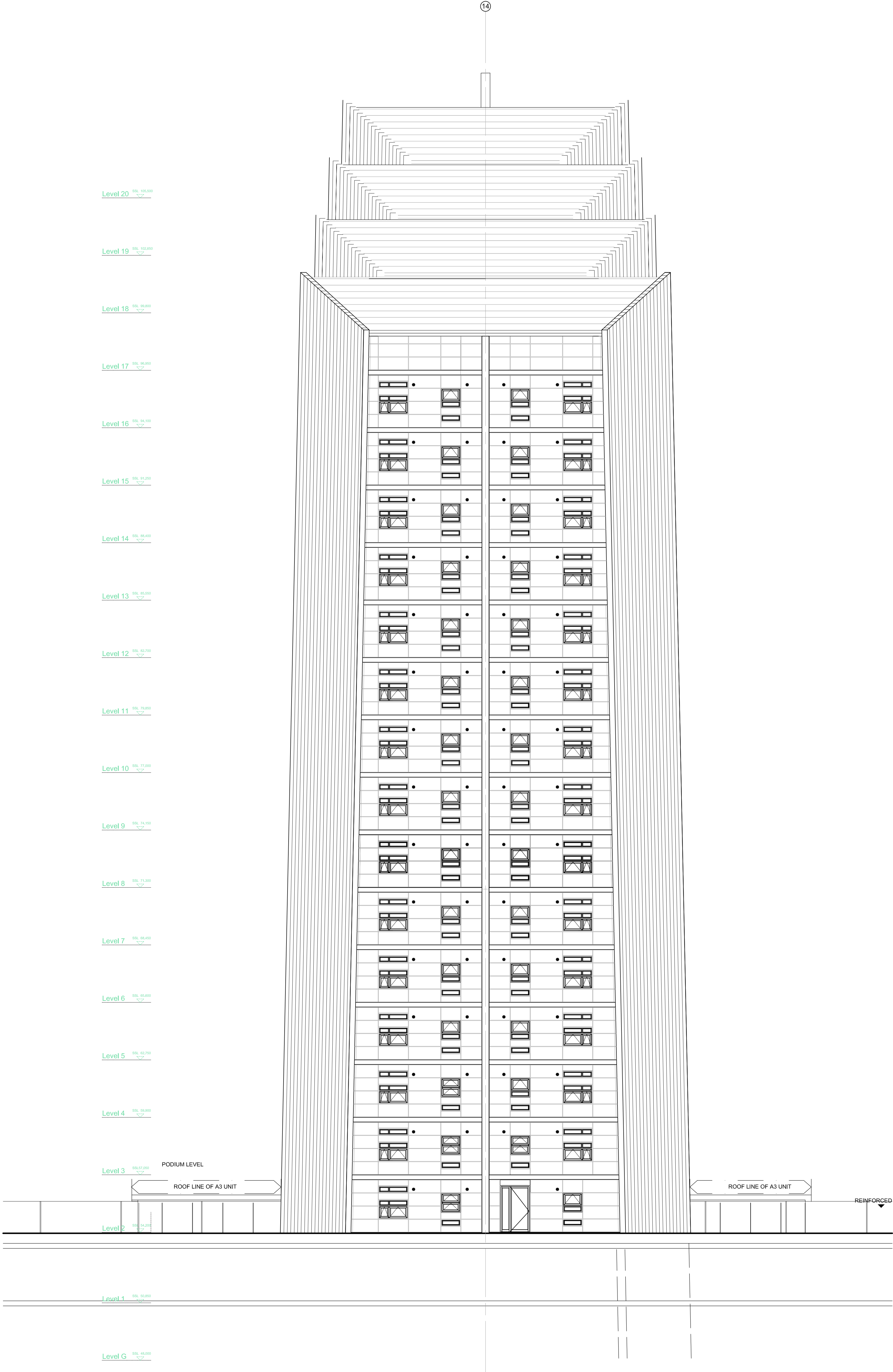
BLOCK B - Elevation B As Proposed
