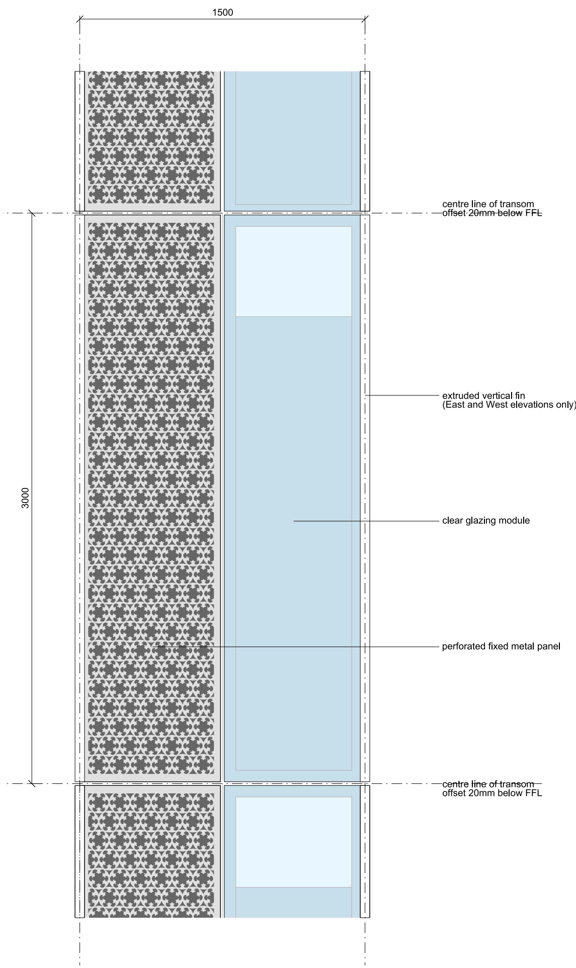
EXTERNAL DETAIL ELEVATION PANEL VENT
