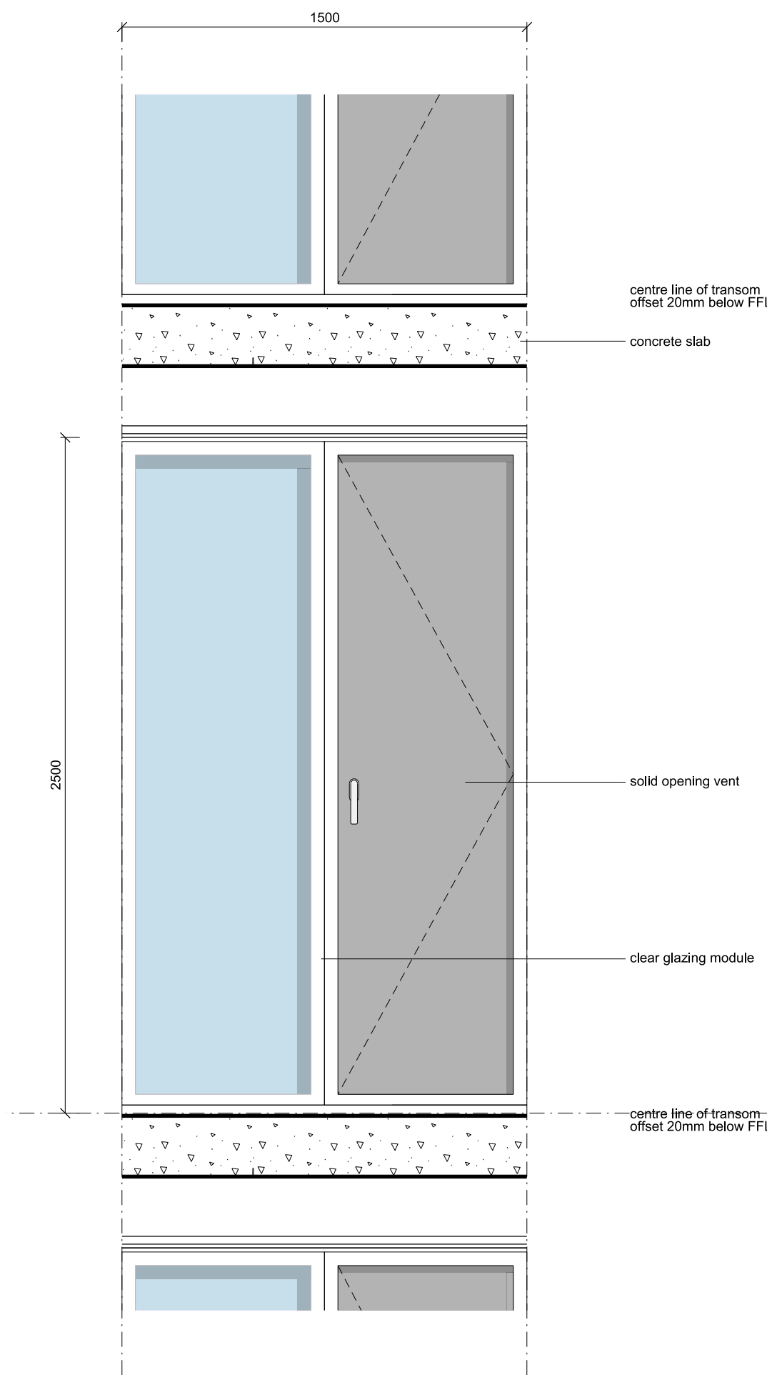
INTERNAL DETAIL ELEVATION PANEL VENT
