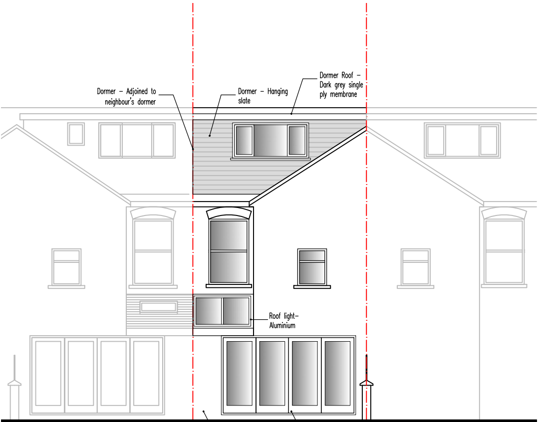
ELEVATION - REAR
