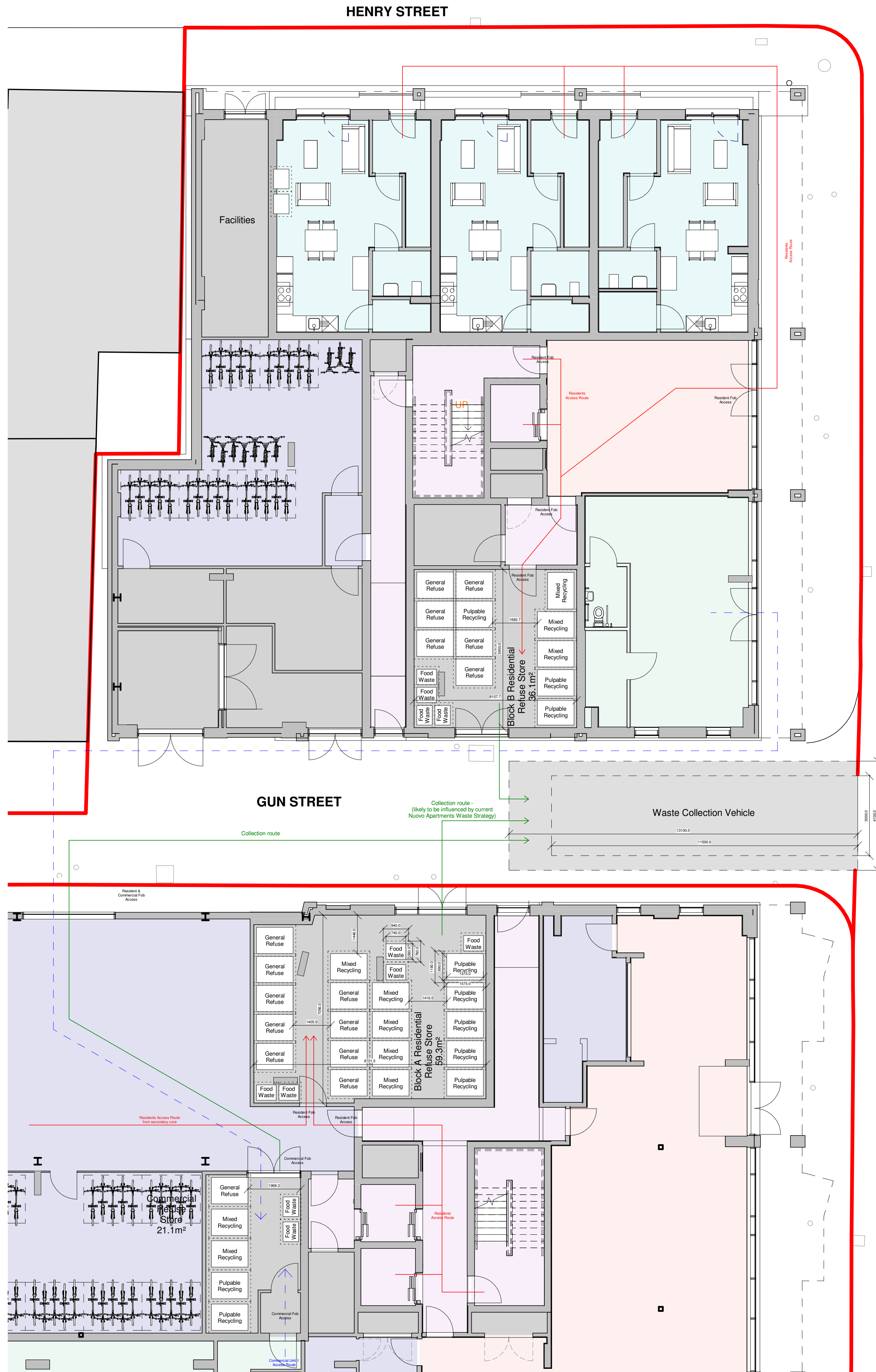
GA_Level 0 Refuse Plan 1 : 100
