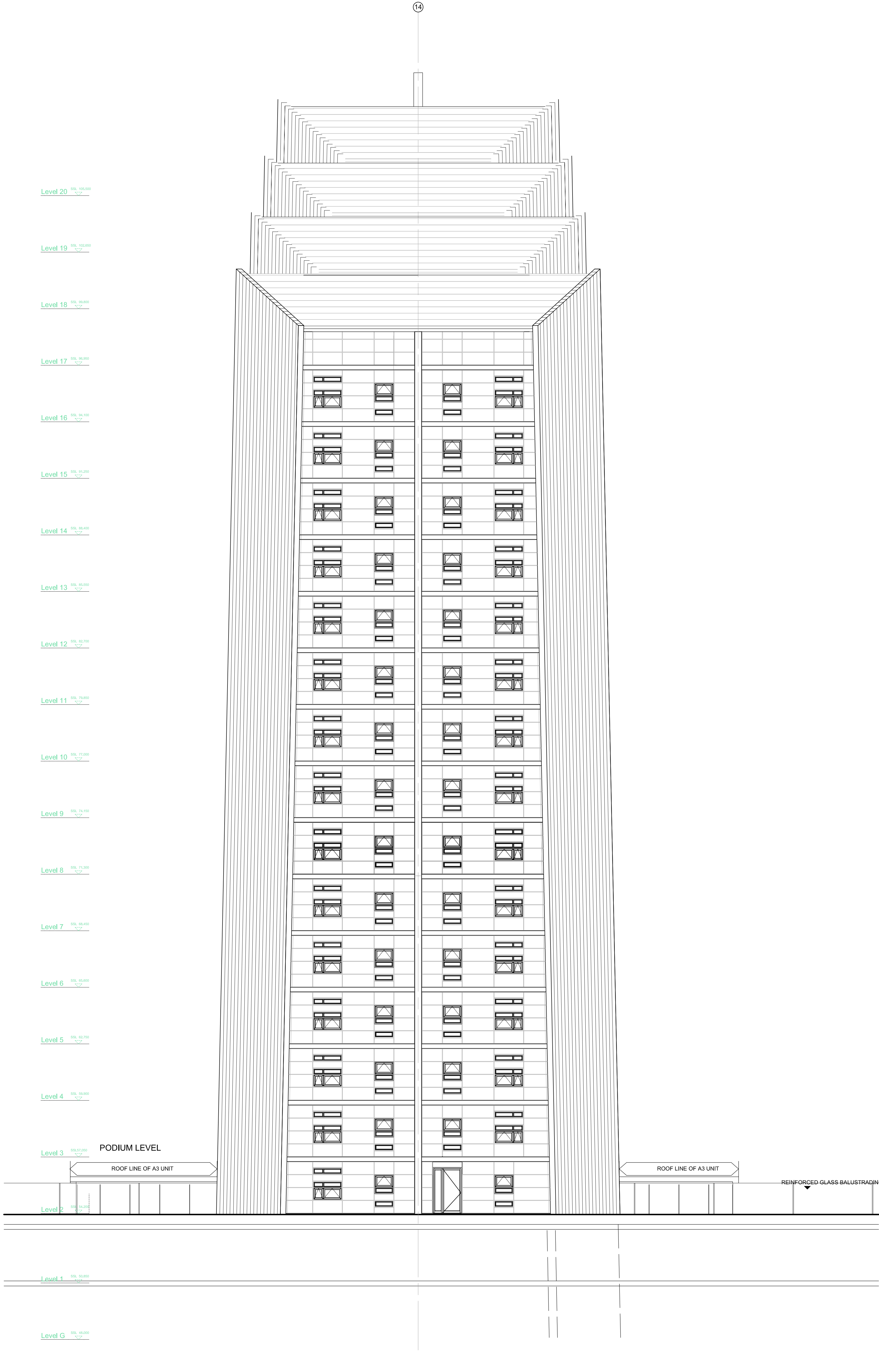
BLOCK B - Elevation B As Existing
