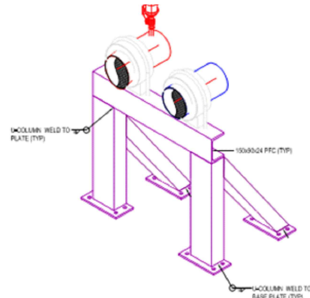
DETAIL 'A' TYPICAL ANCHOR SUPPORT (NTS)
