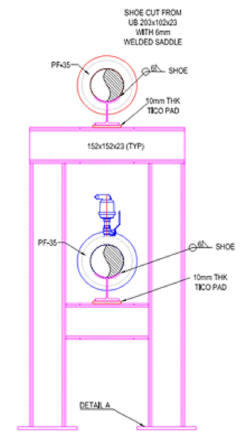
DETAIL 'B' TYPICAL PIPEWORK SUPPORT (NTS)
