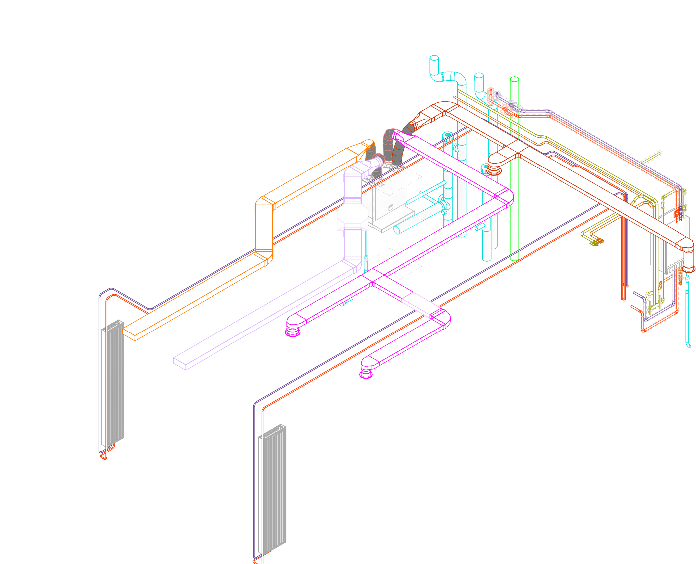
7 TL - COORDINATED SERVICES - TYPICAL 1 BED LEVEL 1 - APARTMENT 1B-TL
