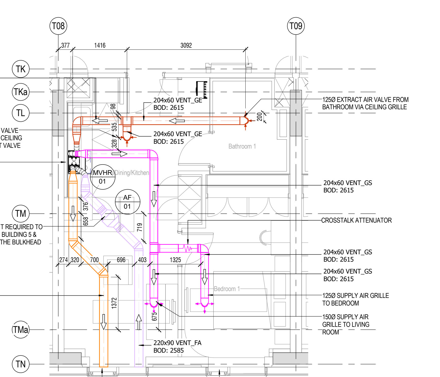
3 TL - VENTILATION - TYPICAL 1 BED LEVEL 1 - APARTMENT 1B-TL
