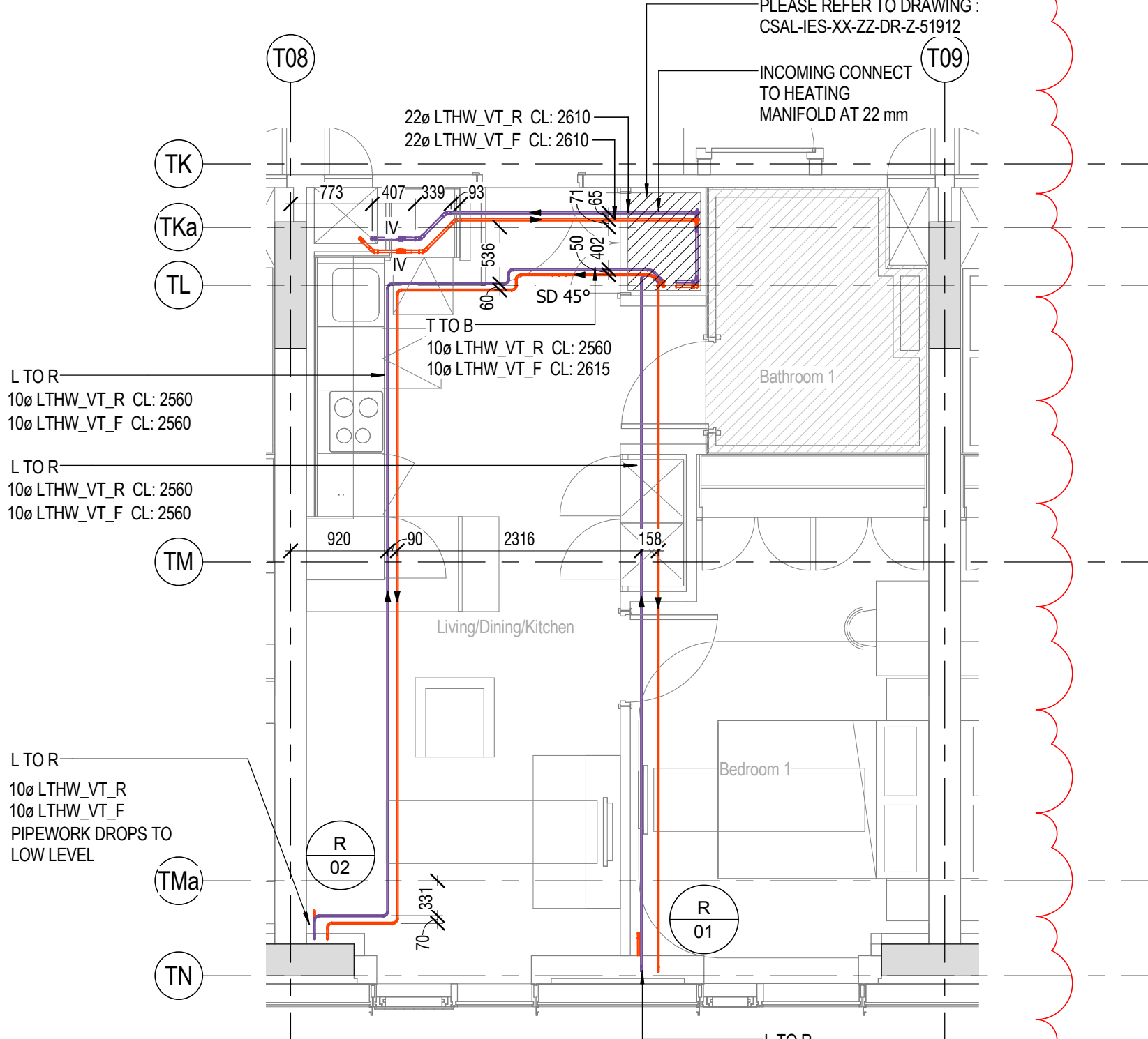
5 TL - HEATING - TYPICAL 1 BED LEVEL 1 - APARTMENT 1B-TL
