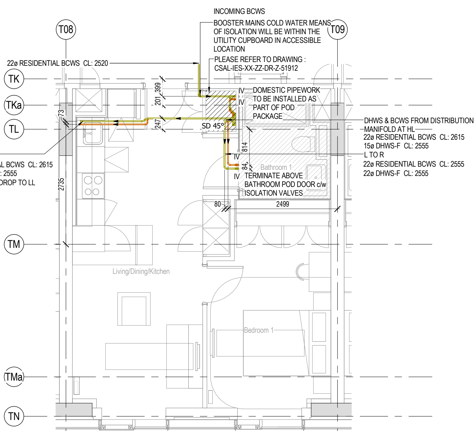
1 TL - DOMESTIC WATER SERVICES - TYPICAL 1 BED LEVEL 1 - APARTMENT 1B-TL
