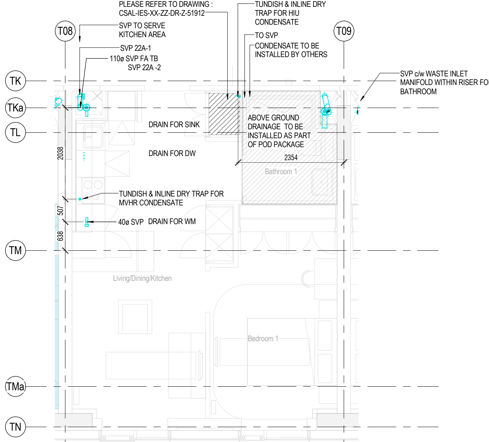
2 TL - ABOVE GROUND DRAINAGE - TYPICAL 1 BED LEVEL 1 - APARTMENT 1B-TL
