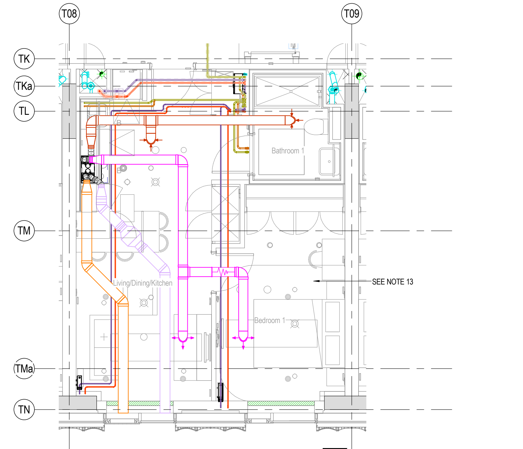
6 TL - COORDINATED SERVICES - TYPICAL 1 BED LEVEL 1 - APARTMENT 1B-TL
