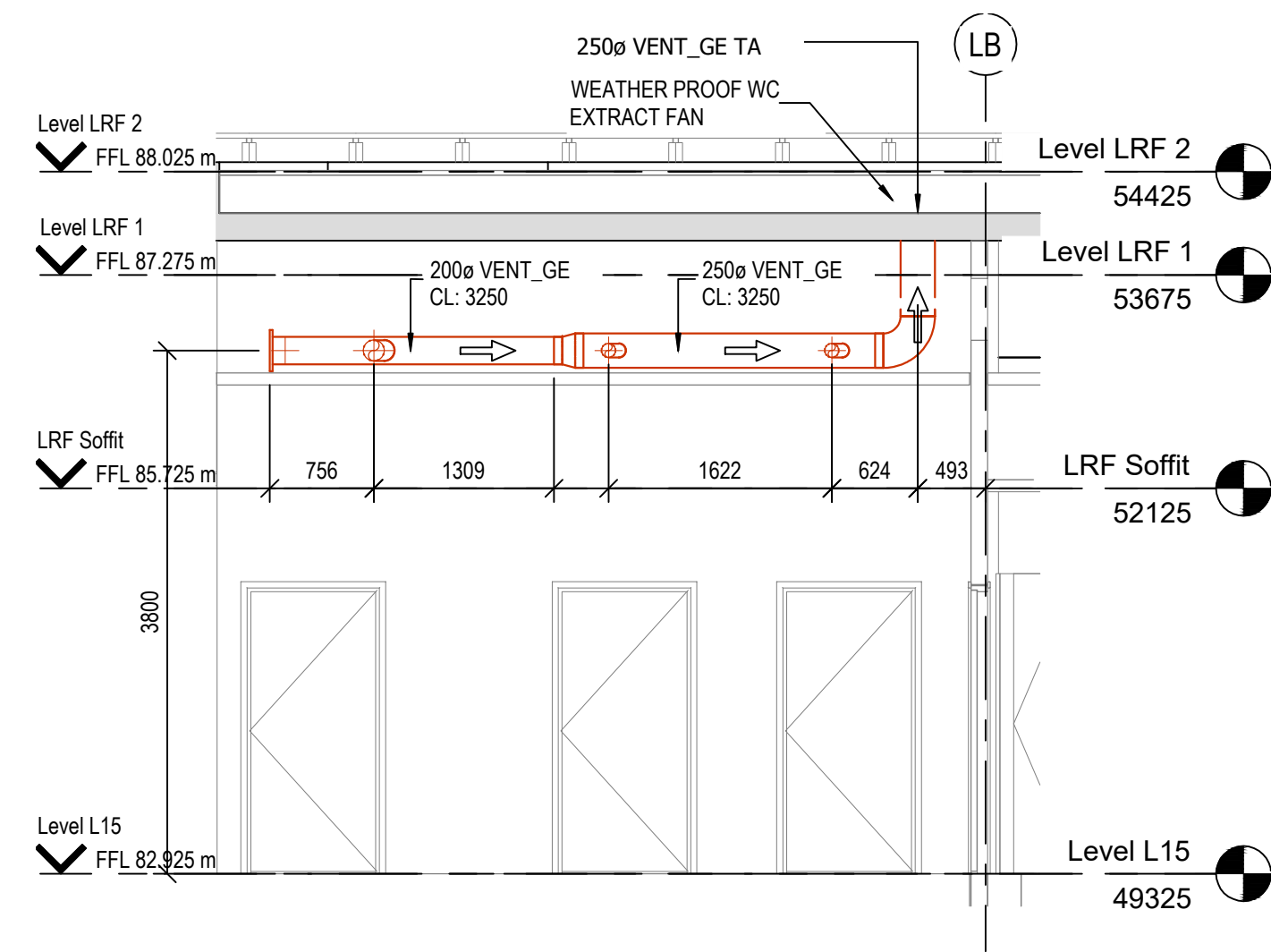
A 7L - VENTILATION - LEVEL 15 - SECTION A 1:50
