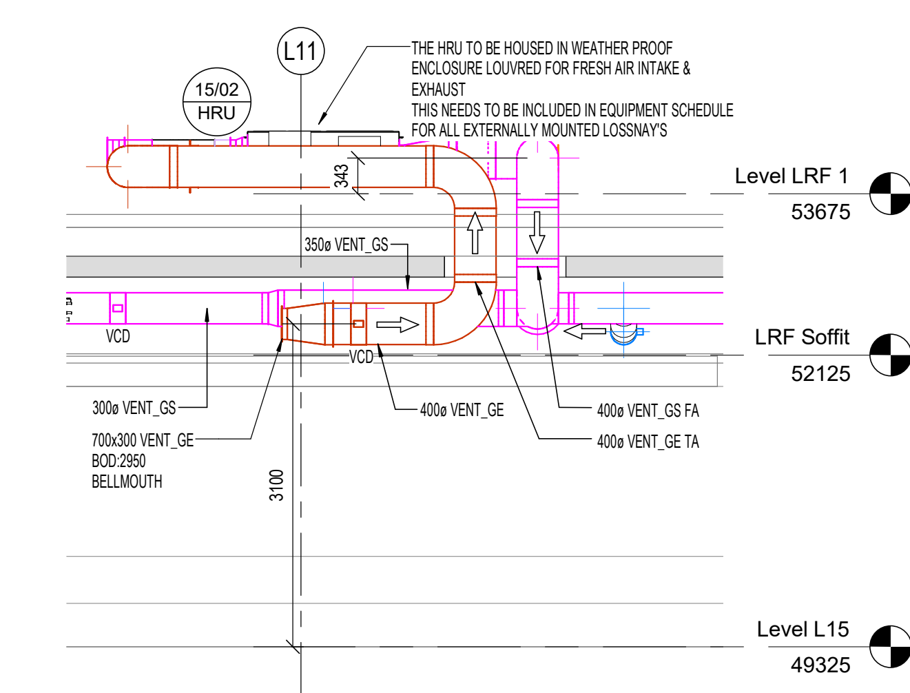
C 8L - VENTILATION - LEVEL 15 - SECTION C 1:50
