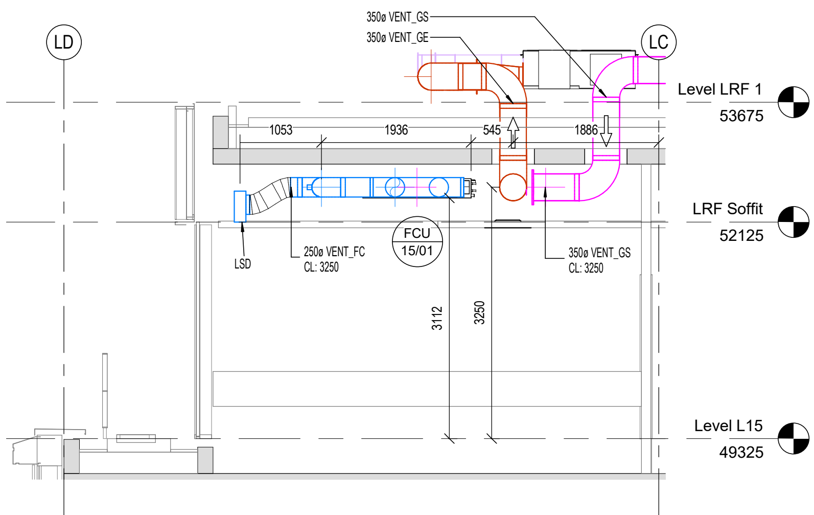
A 8L - VENTILATION - LEVEL 15 - SECTION A 1:50
