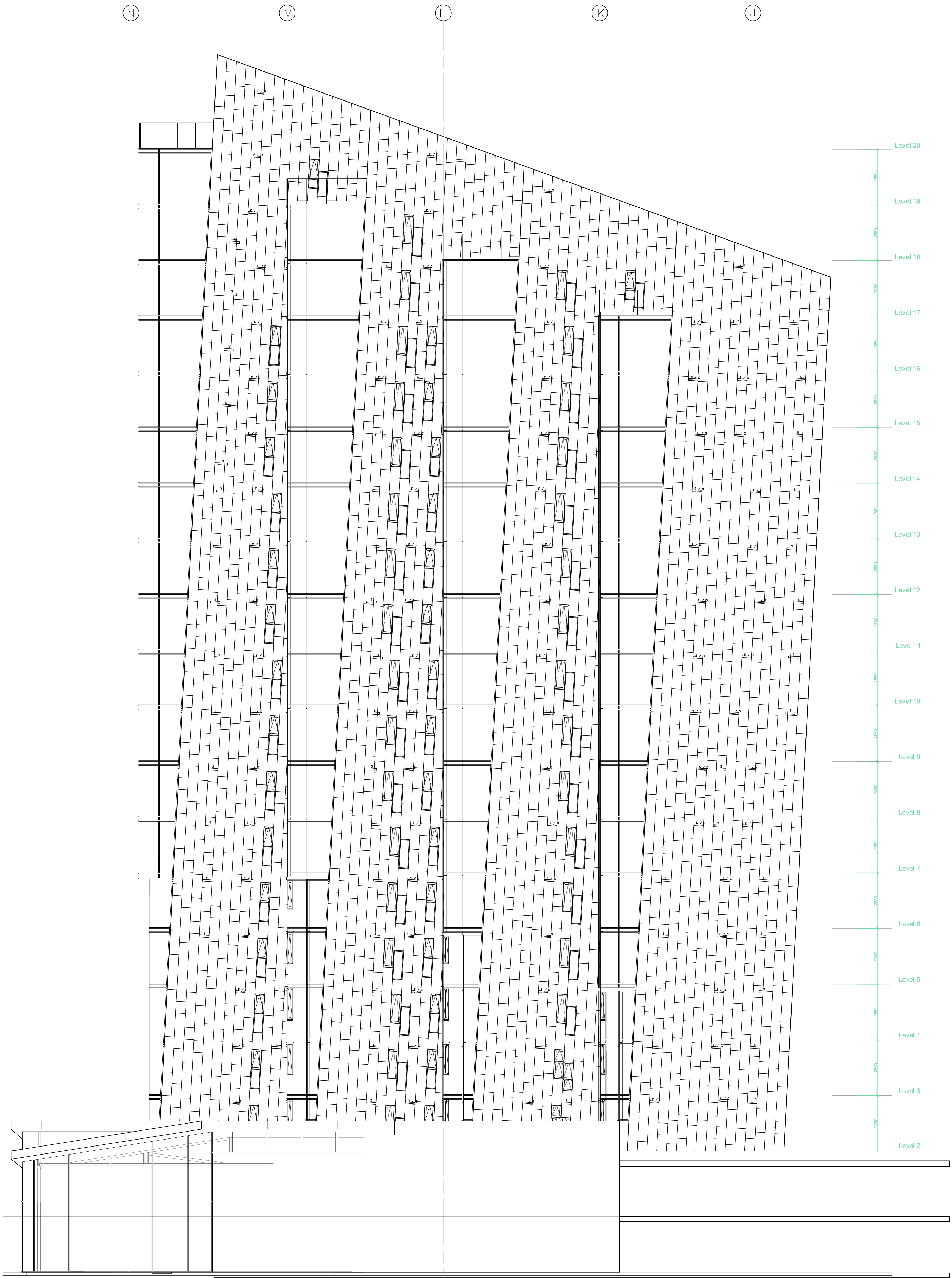
BLOCK B - Elevation C as proposed
