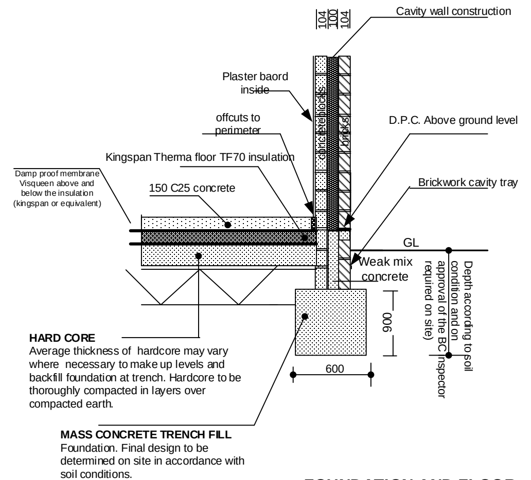
FOUNDATION AND FLOOR Detail
