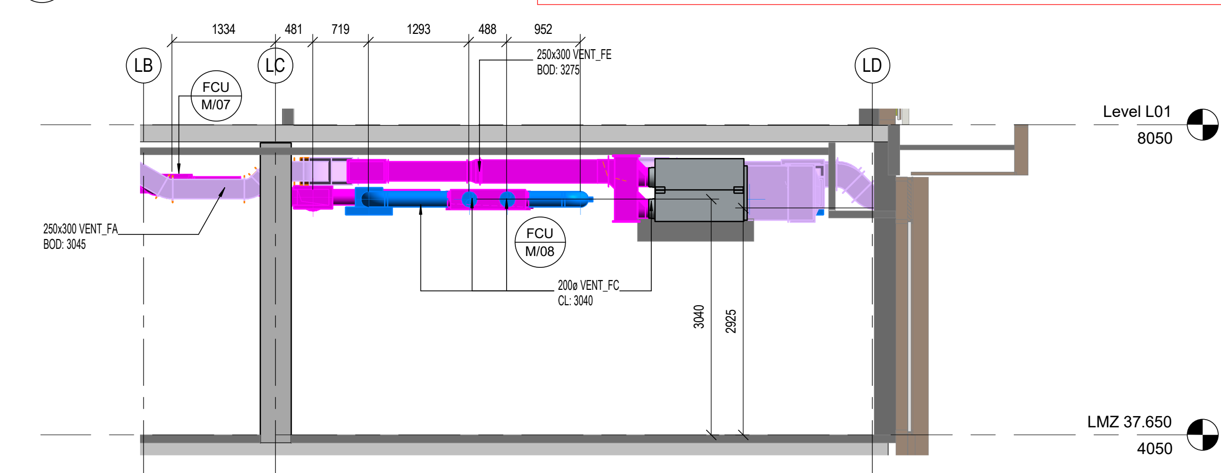
7L - VENTILATION - LEVEL MEZZANINE 1:50
