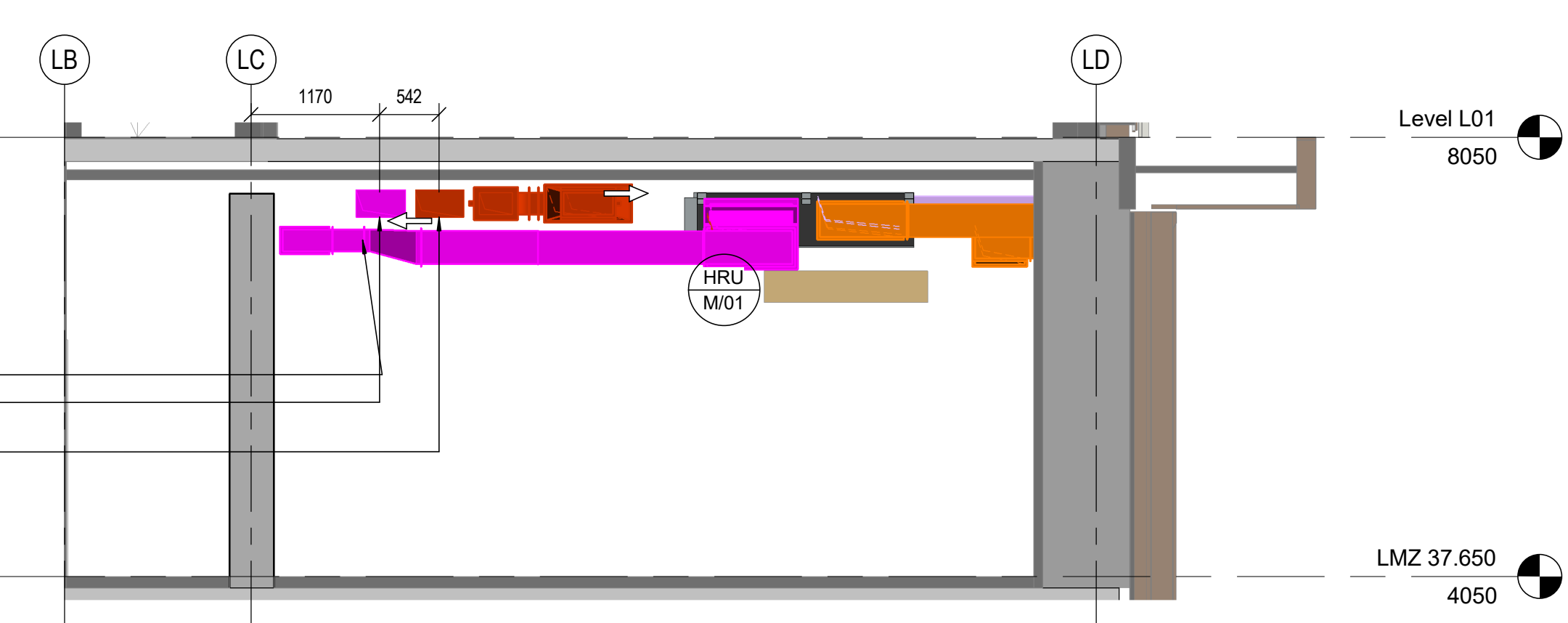
7L - VENTILATION - LEVEL MEZZANINE FLOOR - SECTION C 1:50
