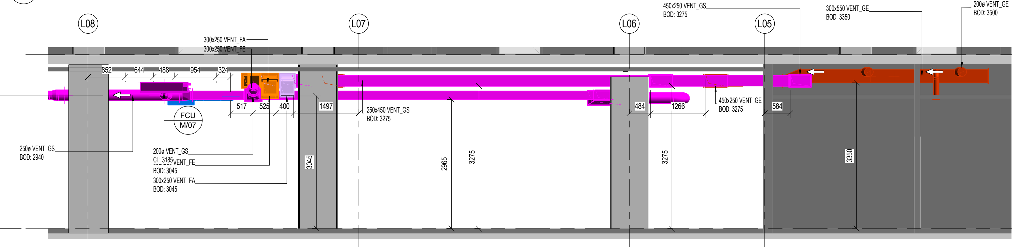
7L - VENTILATION - LEVEL MEZZANINE FLOOR - SECTION B 1:50
