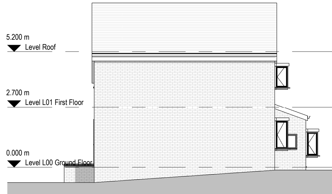
2 Existing West Elevation 1 : 100
