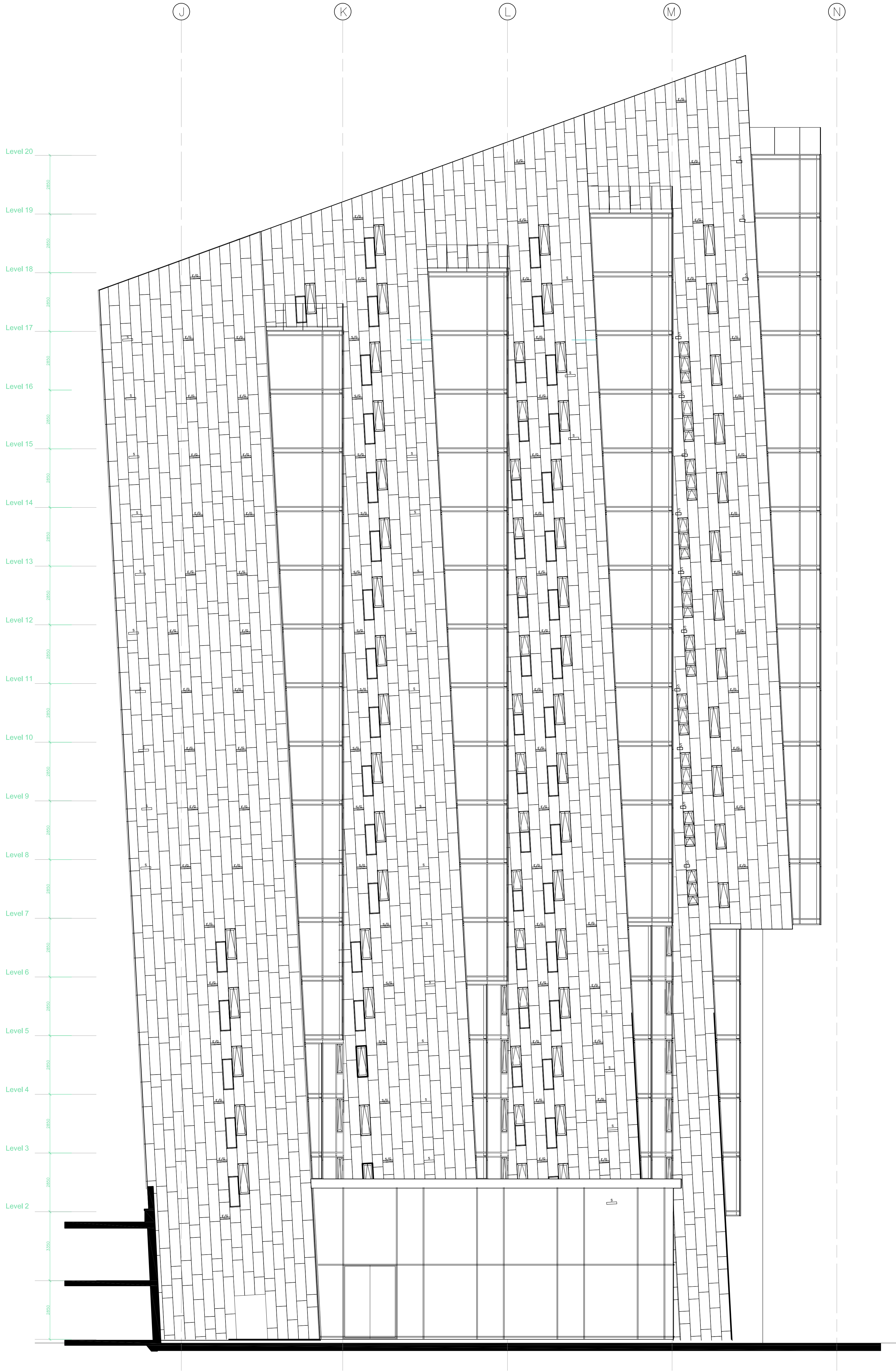
BLOCK B - Elevation A As Proposed
