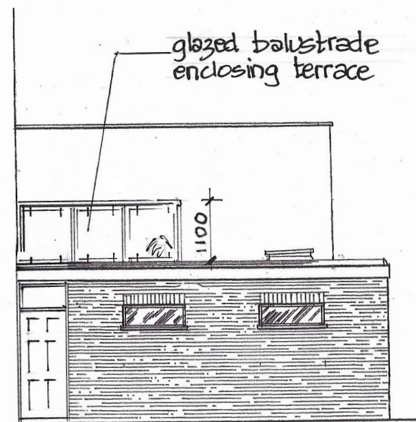
ENTRANCE ELEVATION
