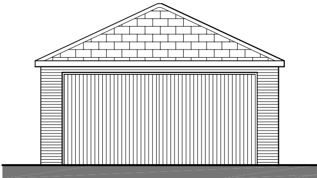
Proposed Front Elevation 1:100
