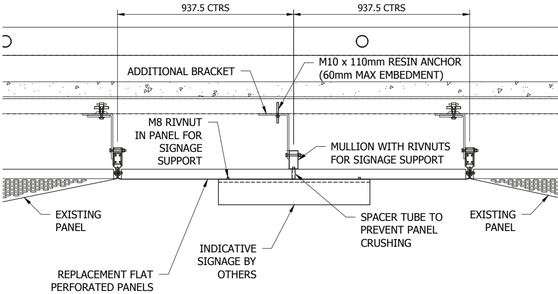
PLAN SECTION A-A
