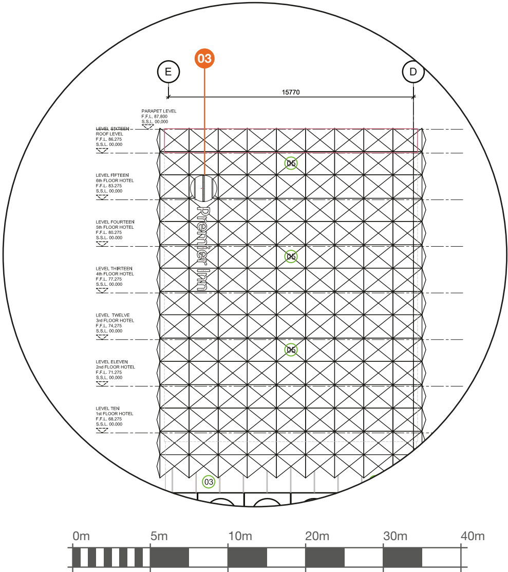
South Elevation - Scale 1:250 @ A3
