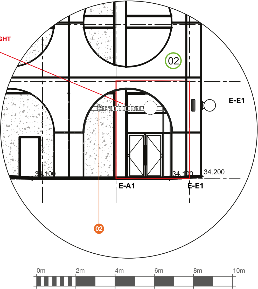
East Elevation - Scale 1:100 @ A3
