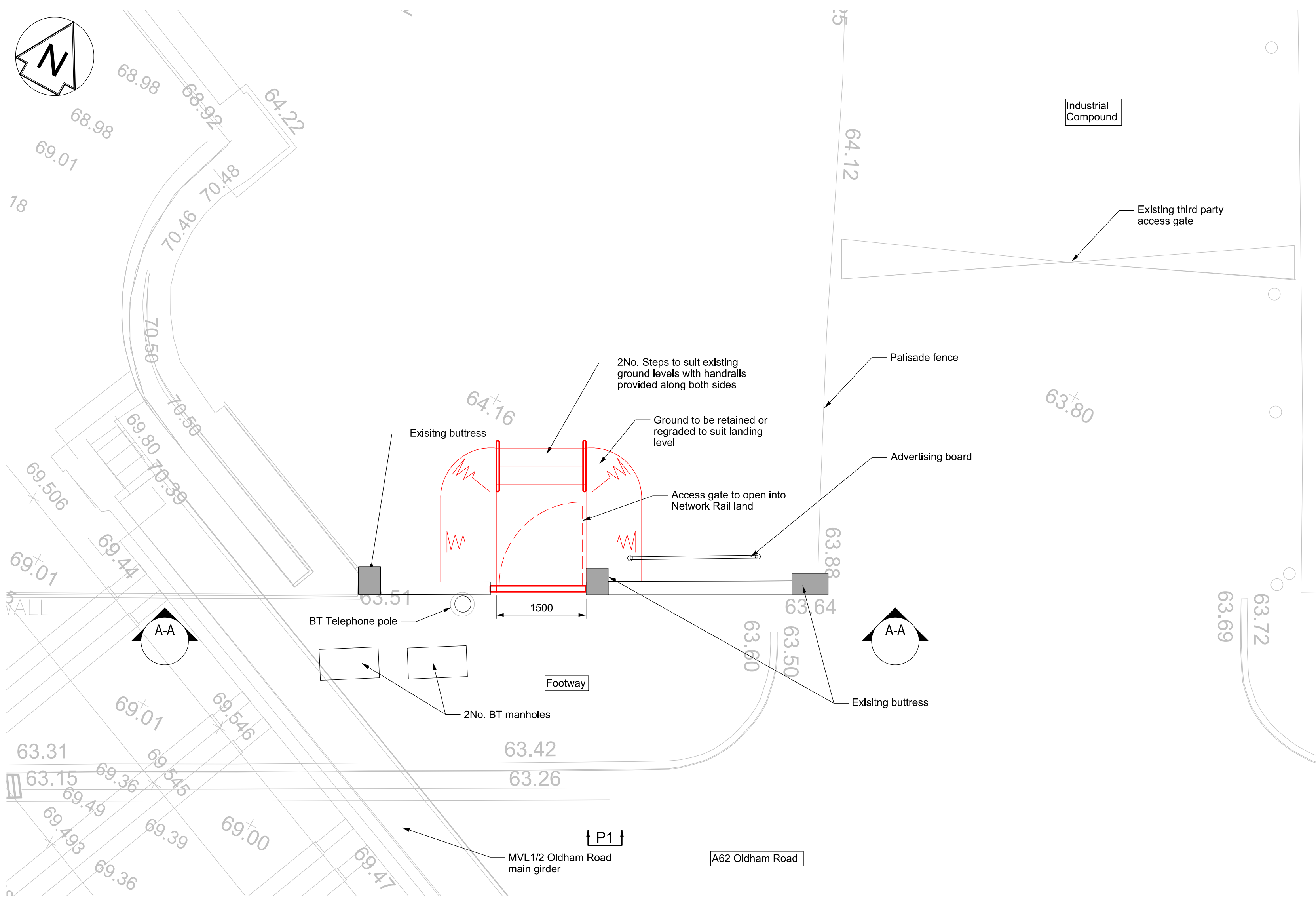
Plan Scale 1:50
