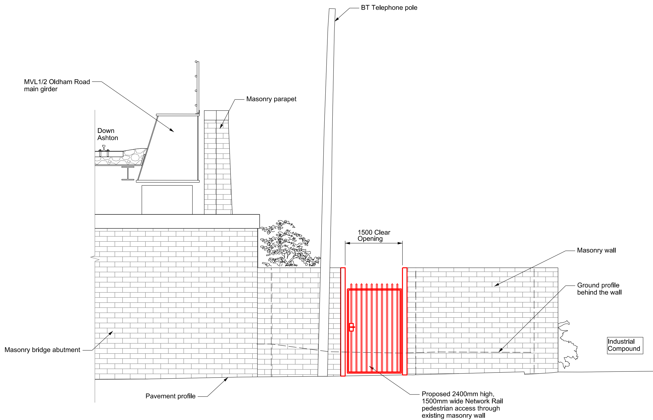
Elevation A-A Scale 1:50
