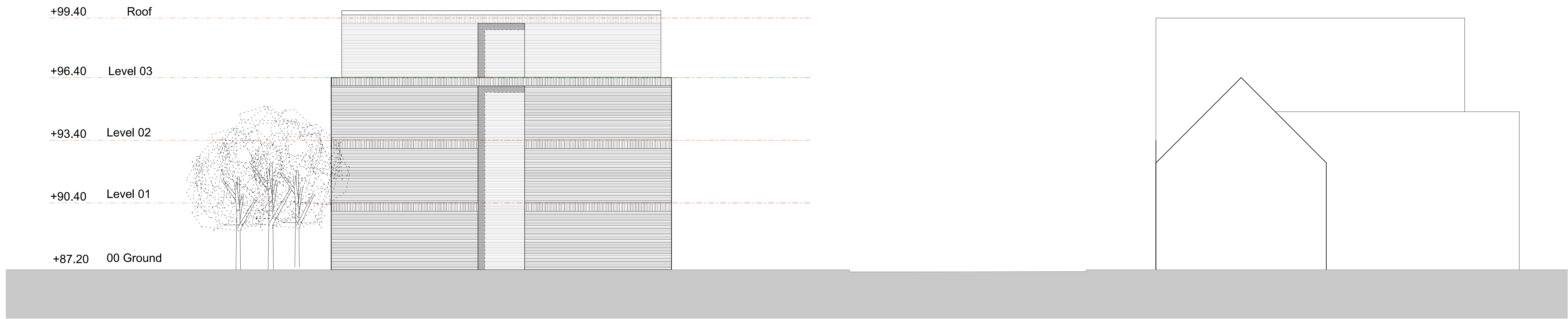
PROPOSED: ELEVATION 04
