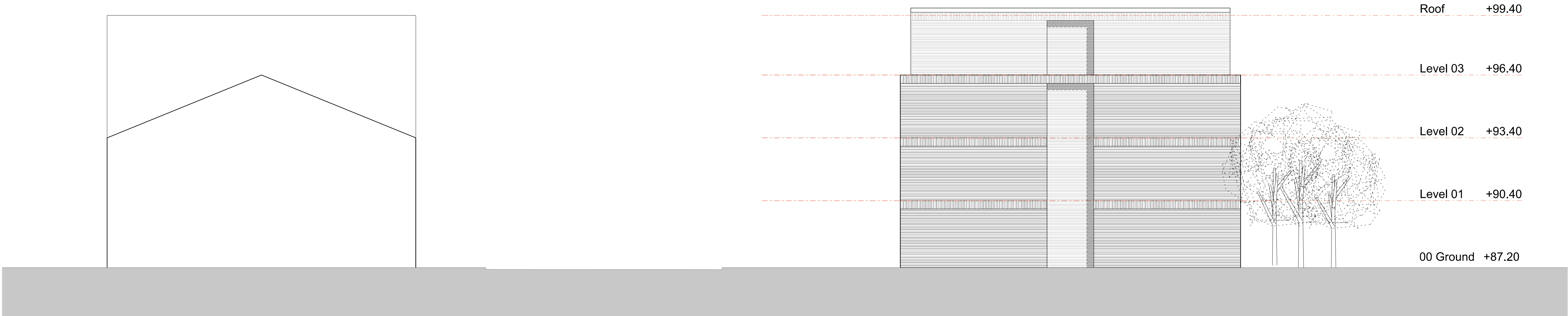
PROPOSED: ELEVATION 03
