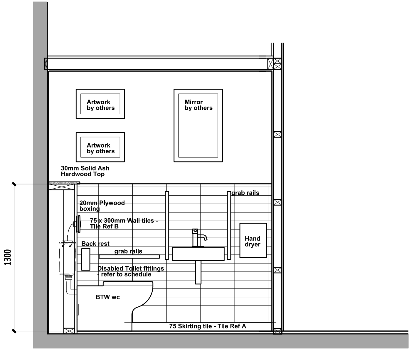
TOILET ELEVATION C 1:20
