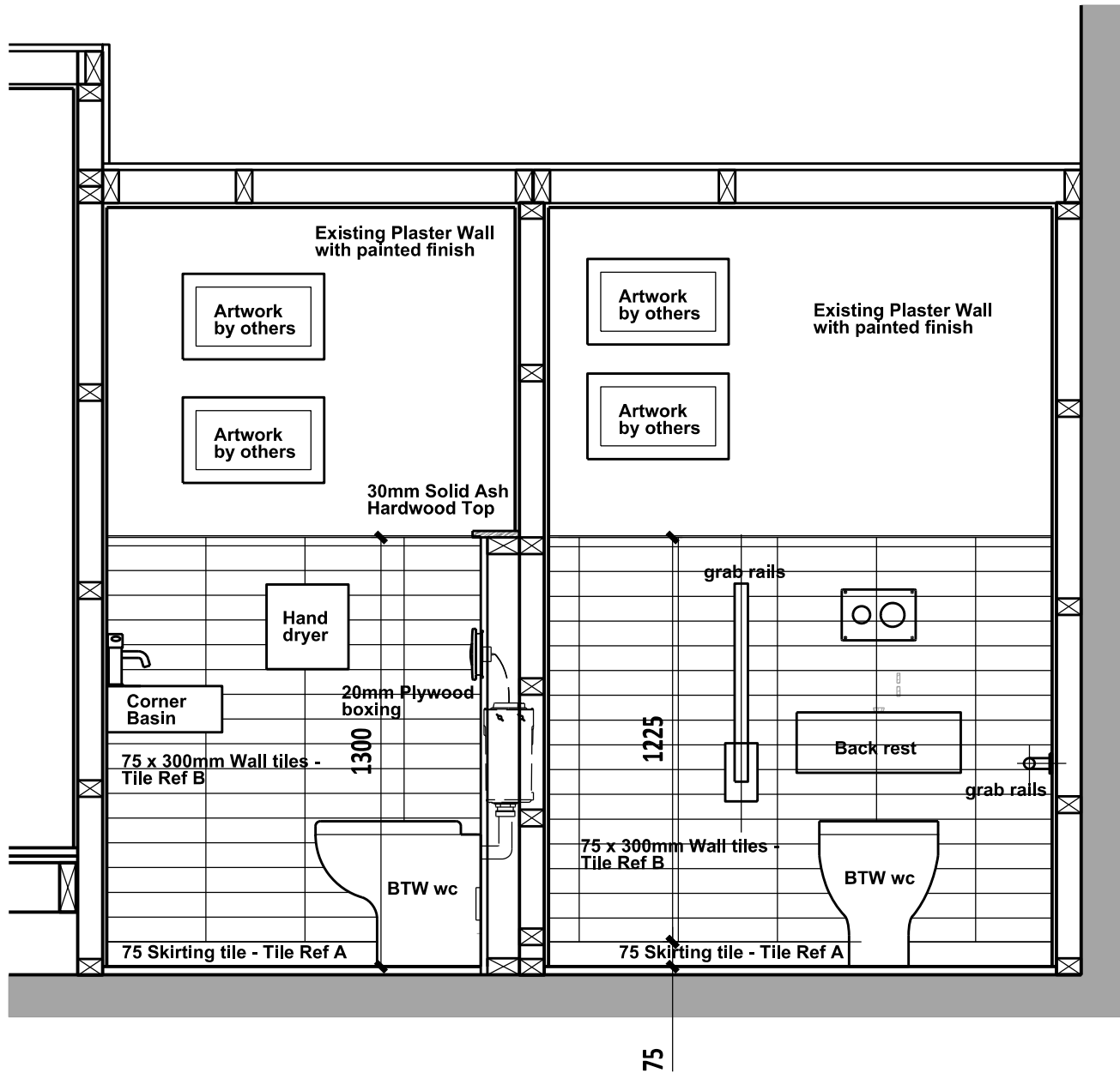
TOILET ELEVATION A 1:20
