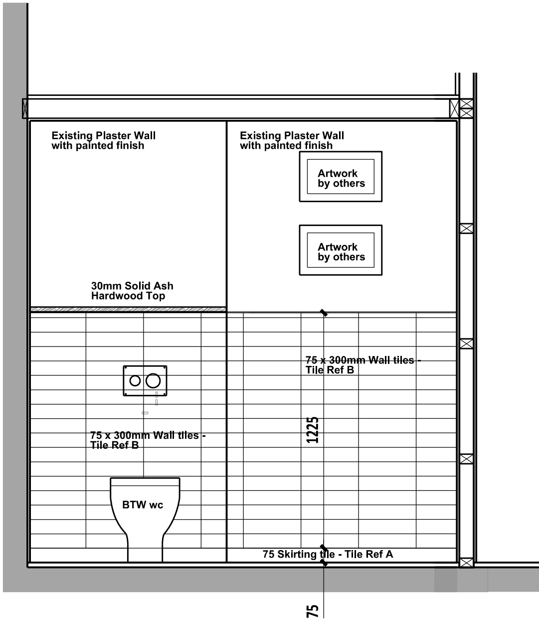
TOILET ELEVATION B 1:20
