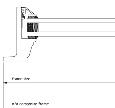
Section F - F
