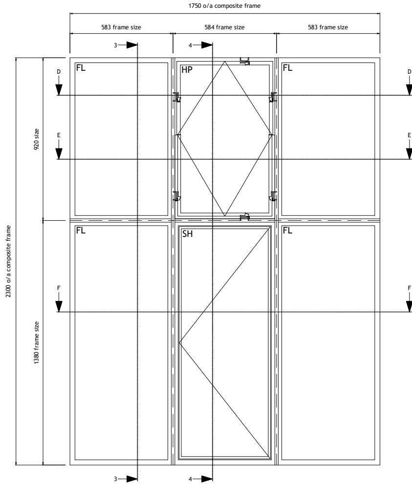
proposed window double glazed
