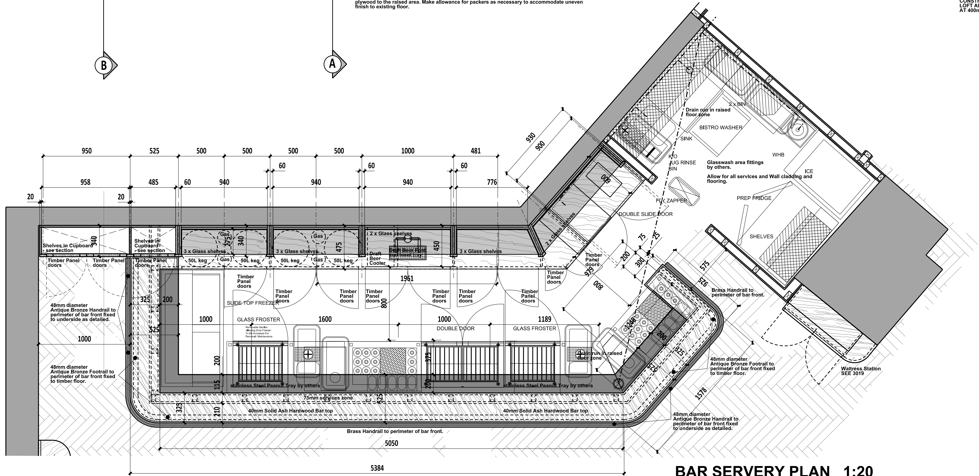
BAR SERVED PLAN 1:20
