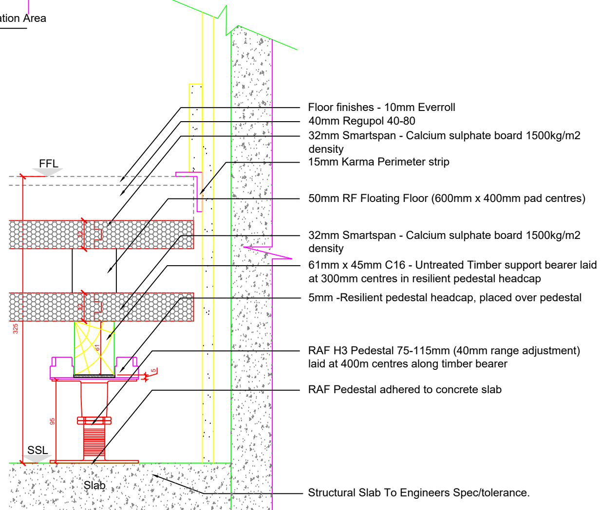
DANSKIN ACOUSTIC FLOOR DETAIL- Gym Area
