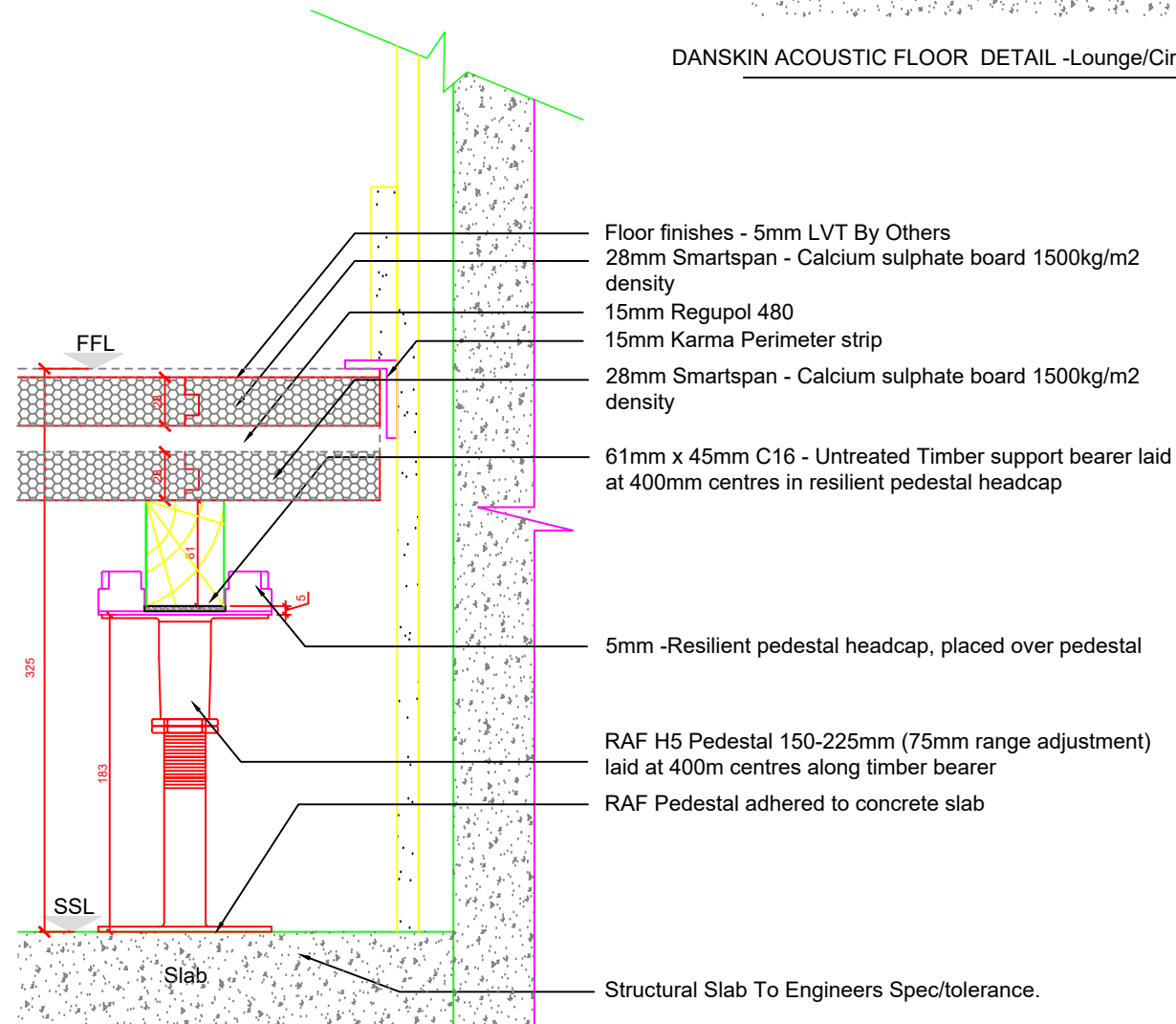
DANSKIN ACOUSTIC FLOOR DETAIL -Studio Area
