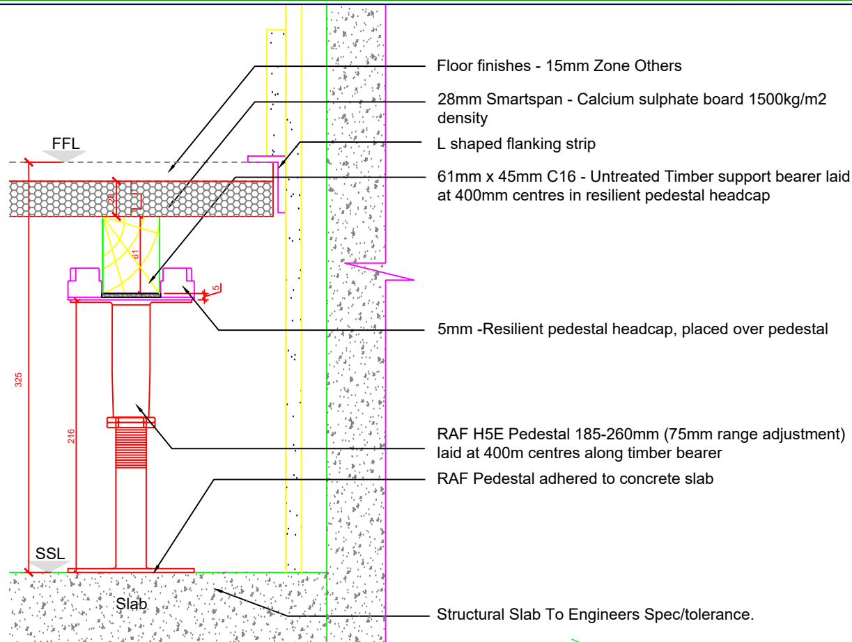
DANSKIN ACOUSTIC FLOOR DETAIL -Lounge/Circulation Area
