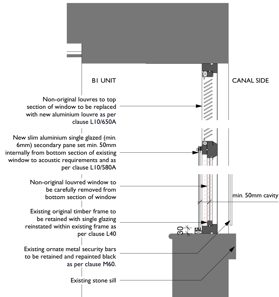
3 Cross Section Detail Scale: 1:10
