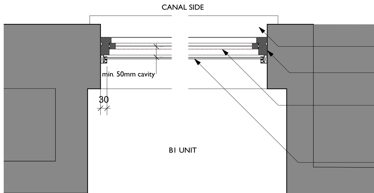
1 Proposed Plan Detail Scale: 1:10
