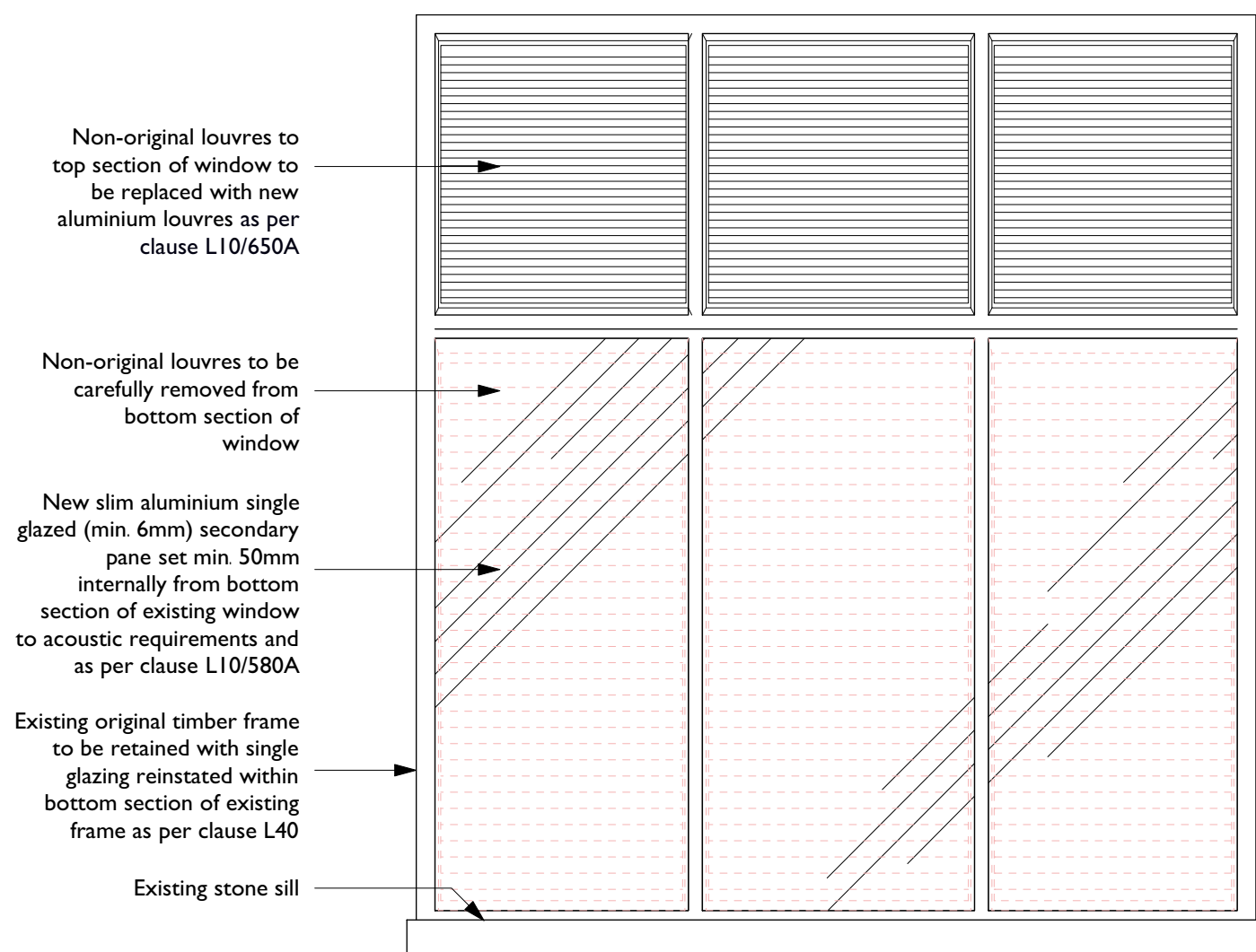
2 Proposed Window Elevation - Exterior Scale: 1:25
