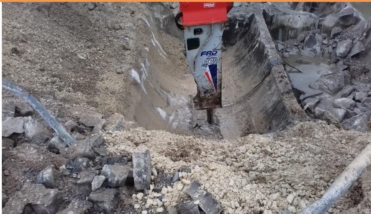
PLATE 8 – PECKING THROUGH BASE OF TANK 2 TO OBTAIN VALIDATION SAMPLE
