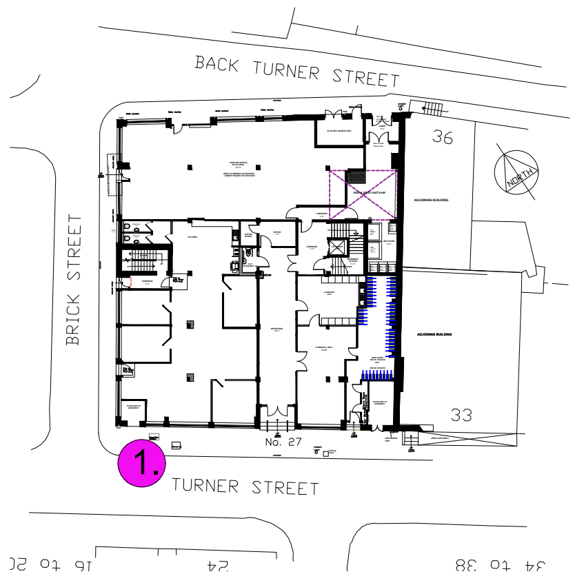
Plan of Location N.T.S.
