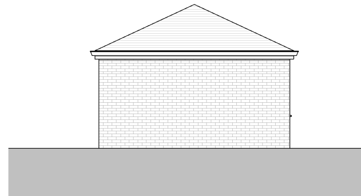
6 Outbuilding West Elevation 1 : 100
