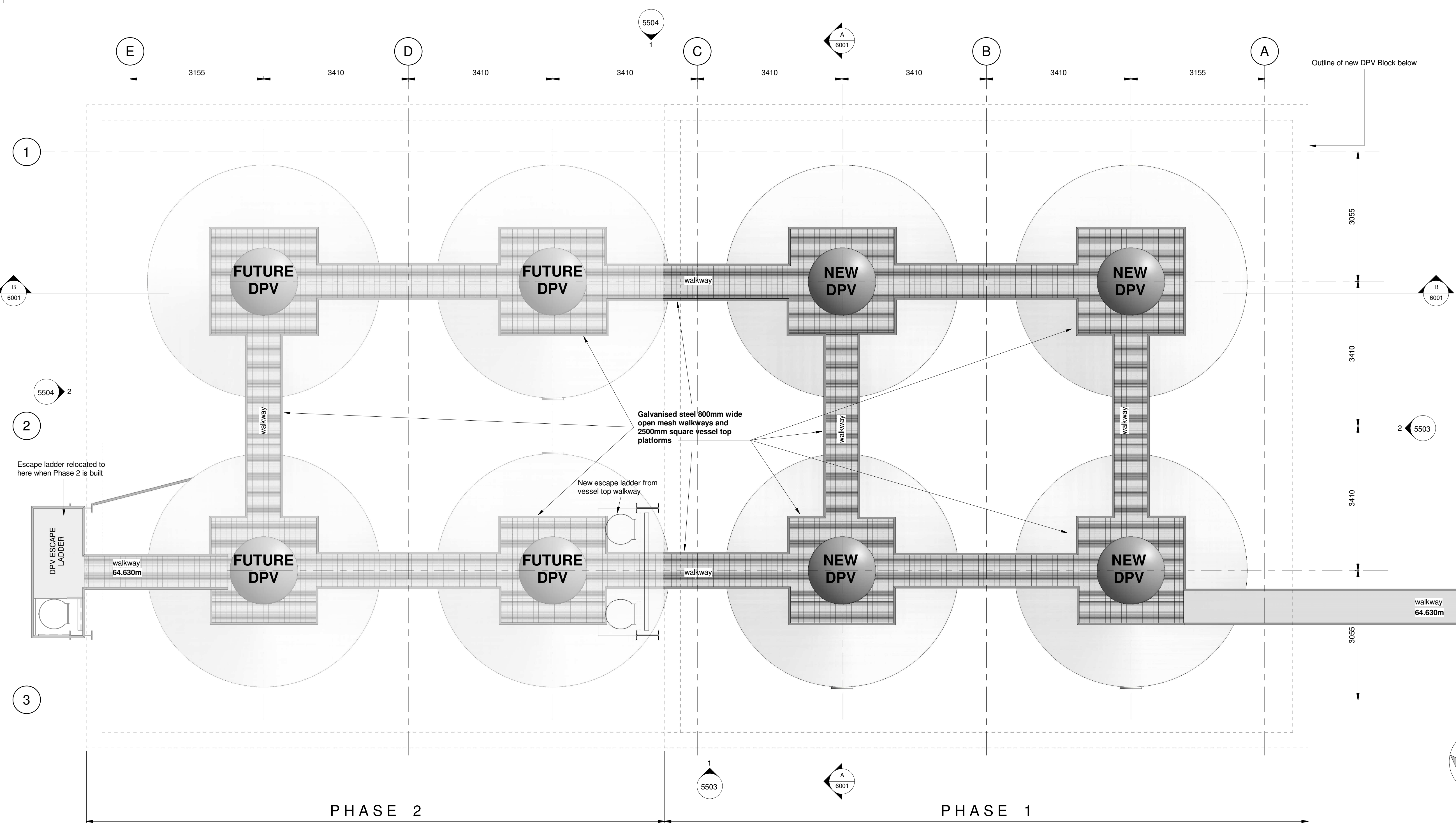
1 DPV Vessel Top Walkway Plan 1 : 50
